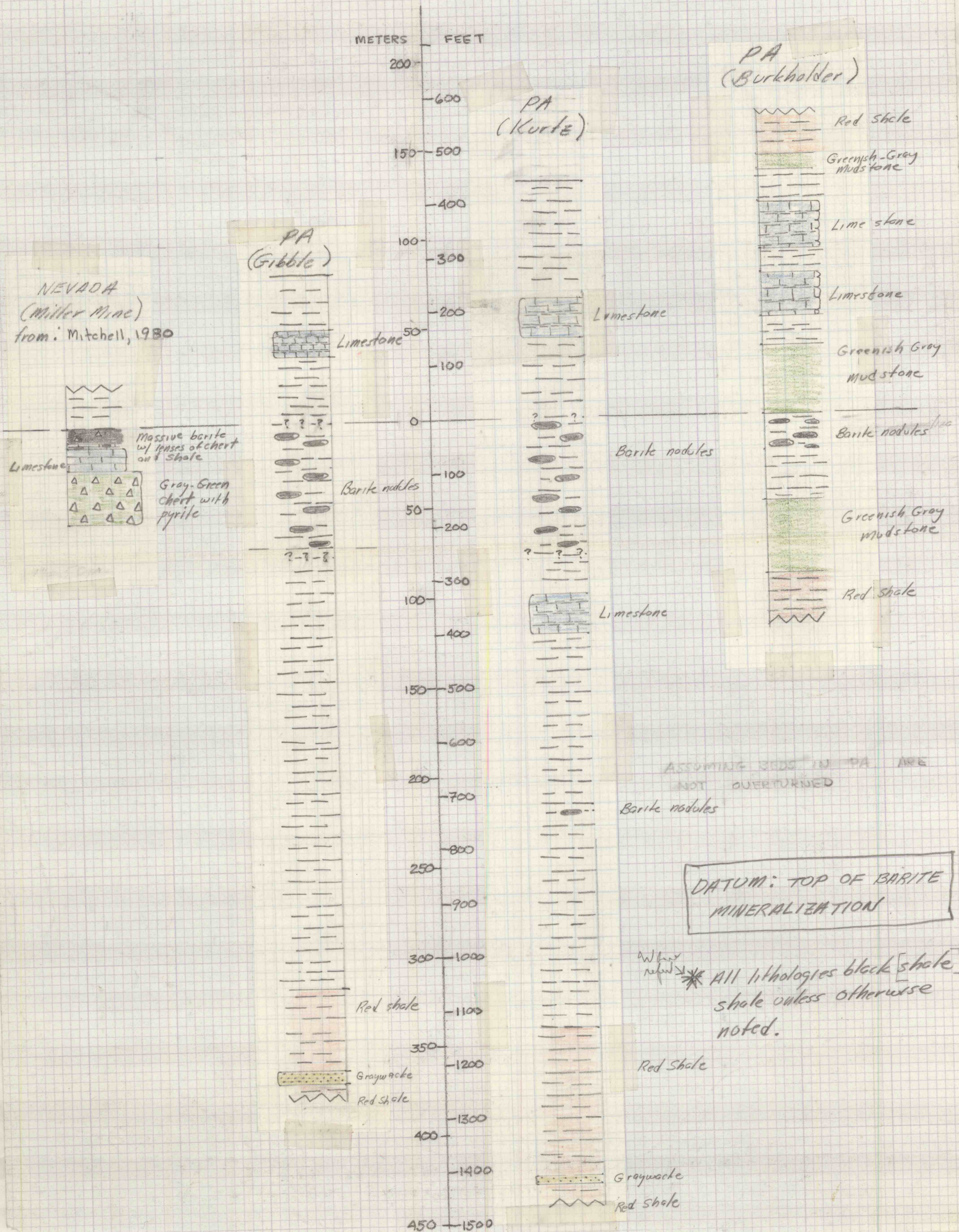
Generalized STRATIGRAPHIC SECTIONS OF SIGNIFICANT MINERALIZED AREAS IN PENNSYLVANIA COMPARED TO A COMMERCIAL DEPOSIT IN NEVADA.
