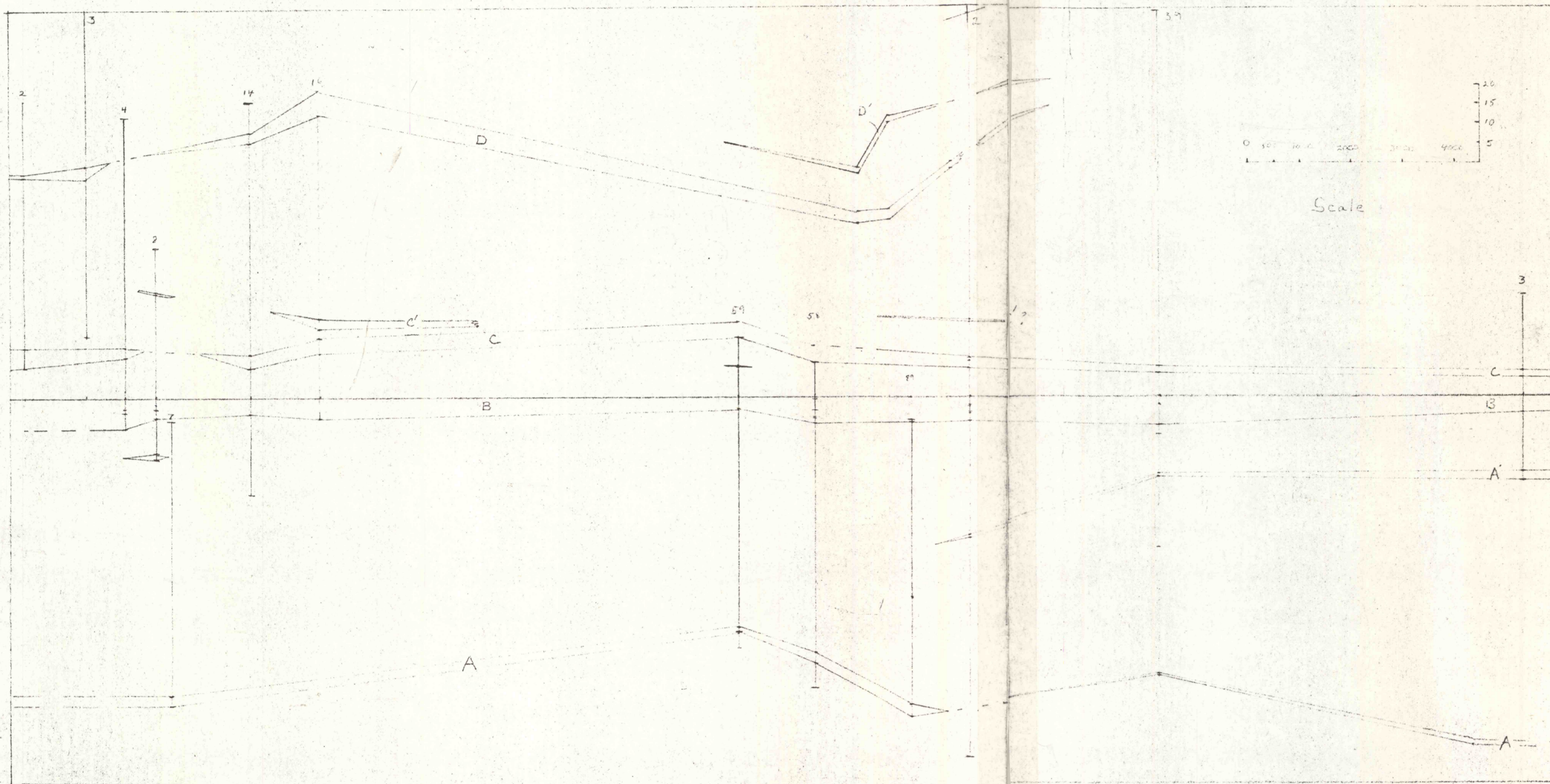
PLATE III COAL CORRELATIONS, BERNICE BASIN. (SEE PLATE I FOR DRILL HOLE LOCATIONS)
