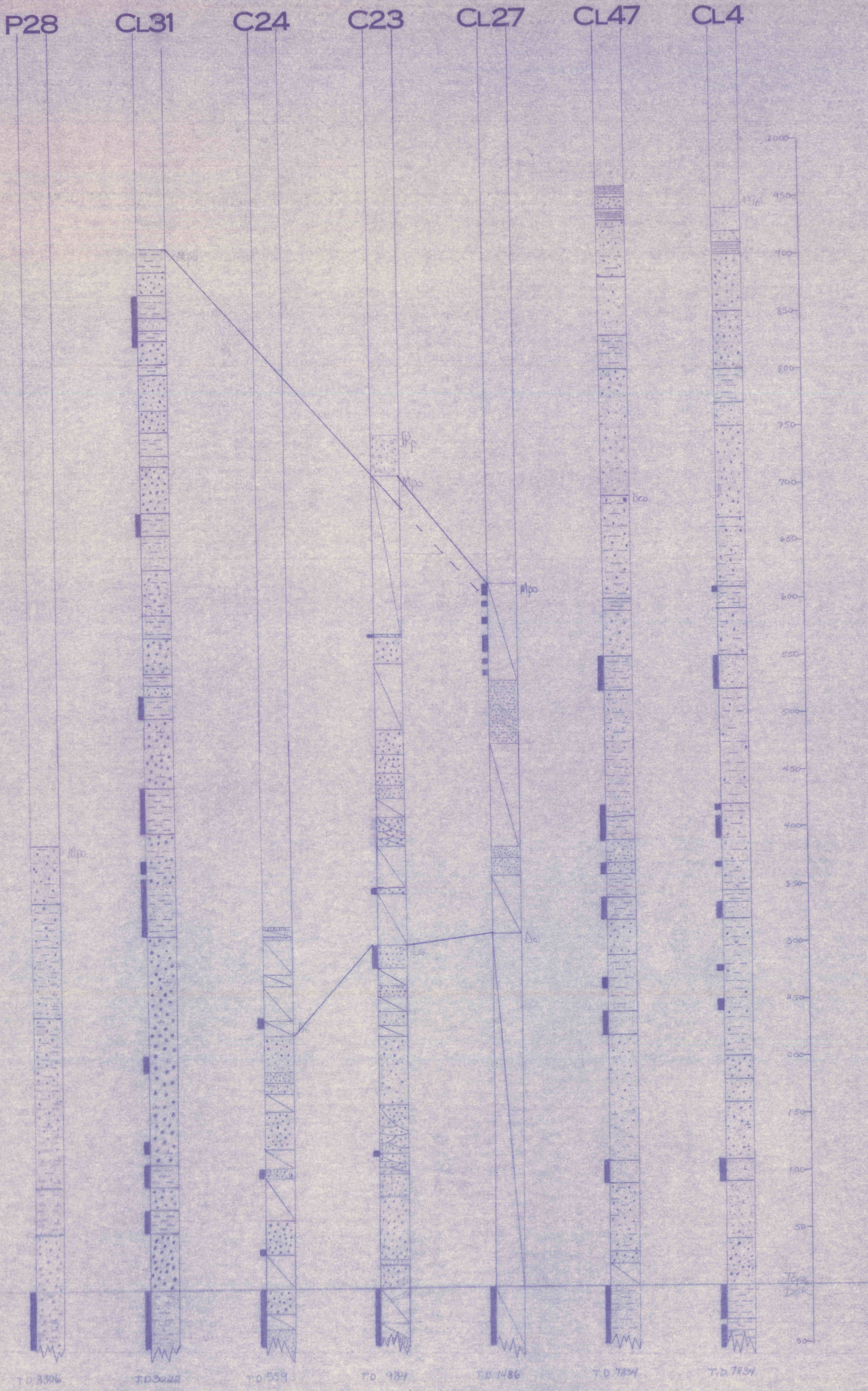
PLATE 5. SECTIONS FROM GEOLOGS SHOWING UPPER DEVONIAN, MISSISSIPPIAN, AND BASAL PENNSYLVANIAN STRATA
