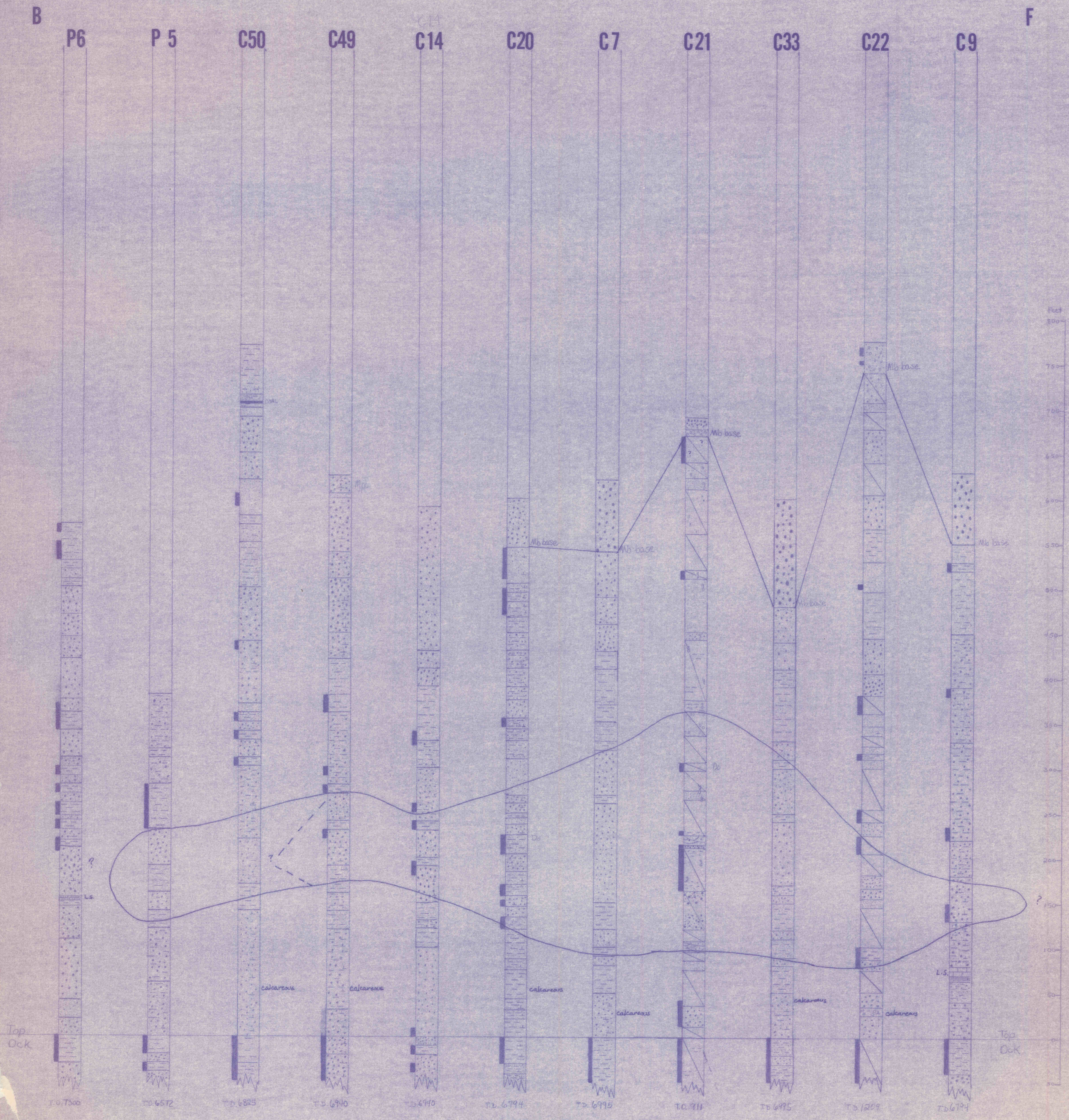
Plate 2. Sections From Geologs Showing Upper Devonian, Mississippian, And Basal Pennsylvanian Strata
