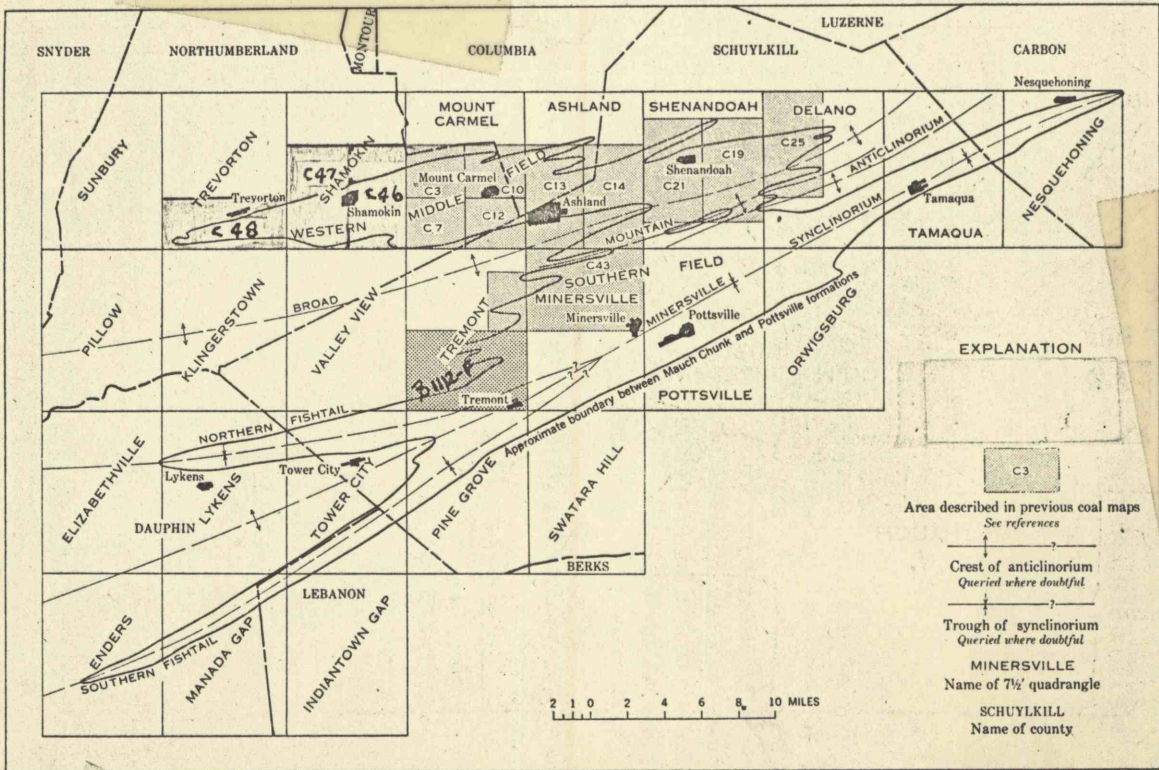
FIGURE 2.—Index map of the Southern and Western Middle anthracite fields showing the location of the mapped area and major structural features.
