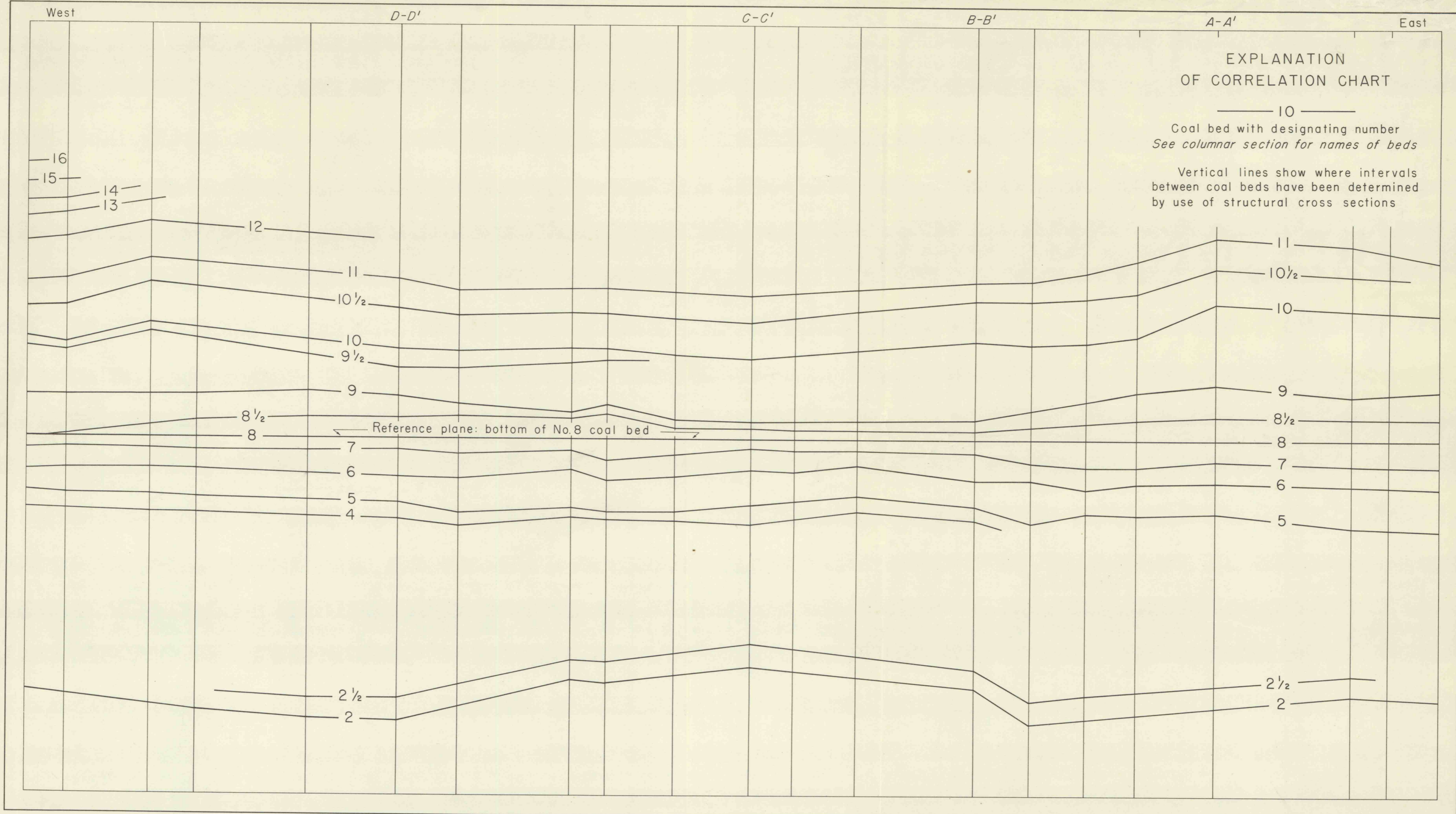
CORRELATION CHART SHOWING THE EAST-WEST LATERAL VARIATION IN THE INTERVALS BETWEEN COAL BEDS IN THE SOUTH LIMB OF THE MAHANOY BASIN
