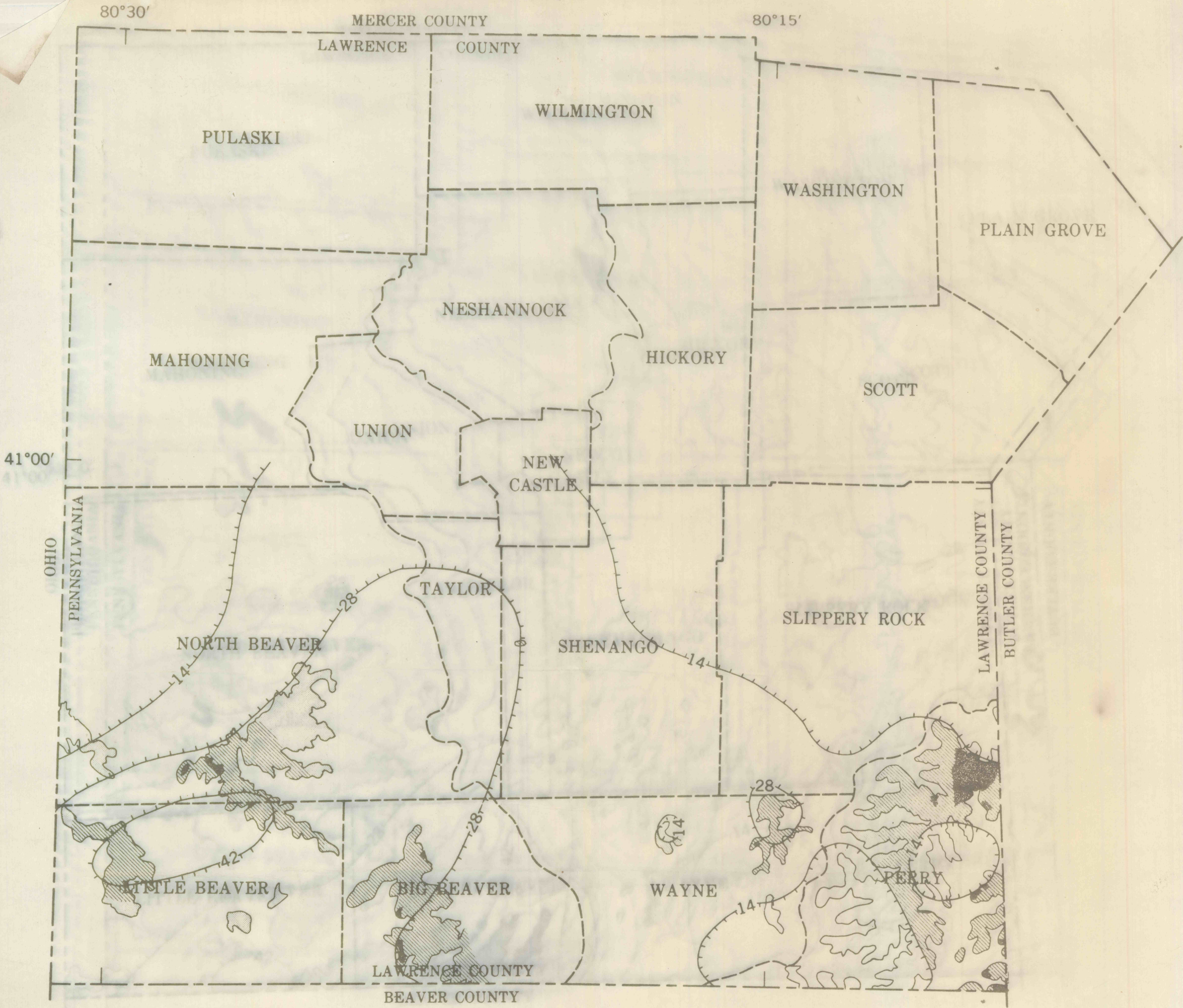
H. LOWER FREEPORT COAL BED
