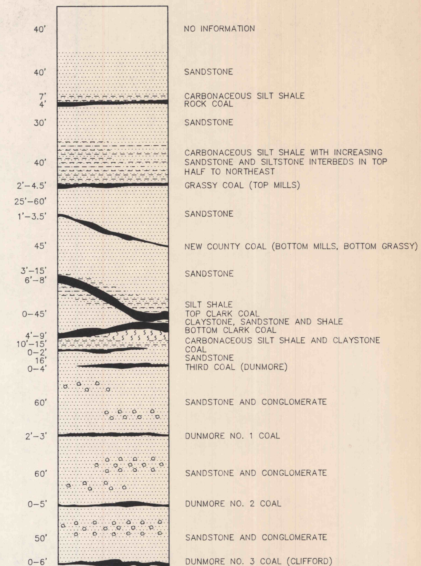
PRELIMINARY STRATIGRAPHIC SECTION OF THE NORTHWEST COLLIERY COAL-BEARING SEQUENCE (LOWER PART OF THE LLEWELLYN FORMATION).
