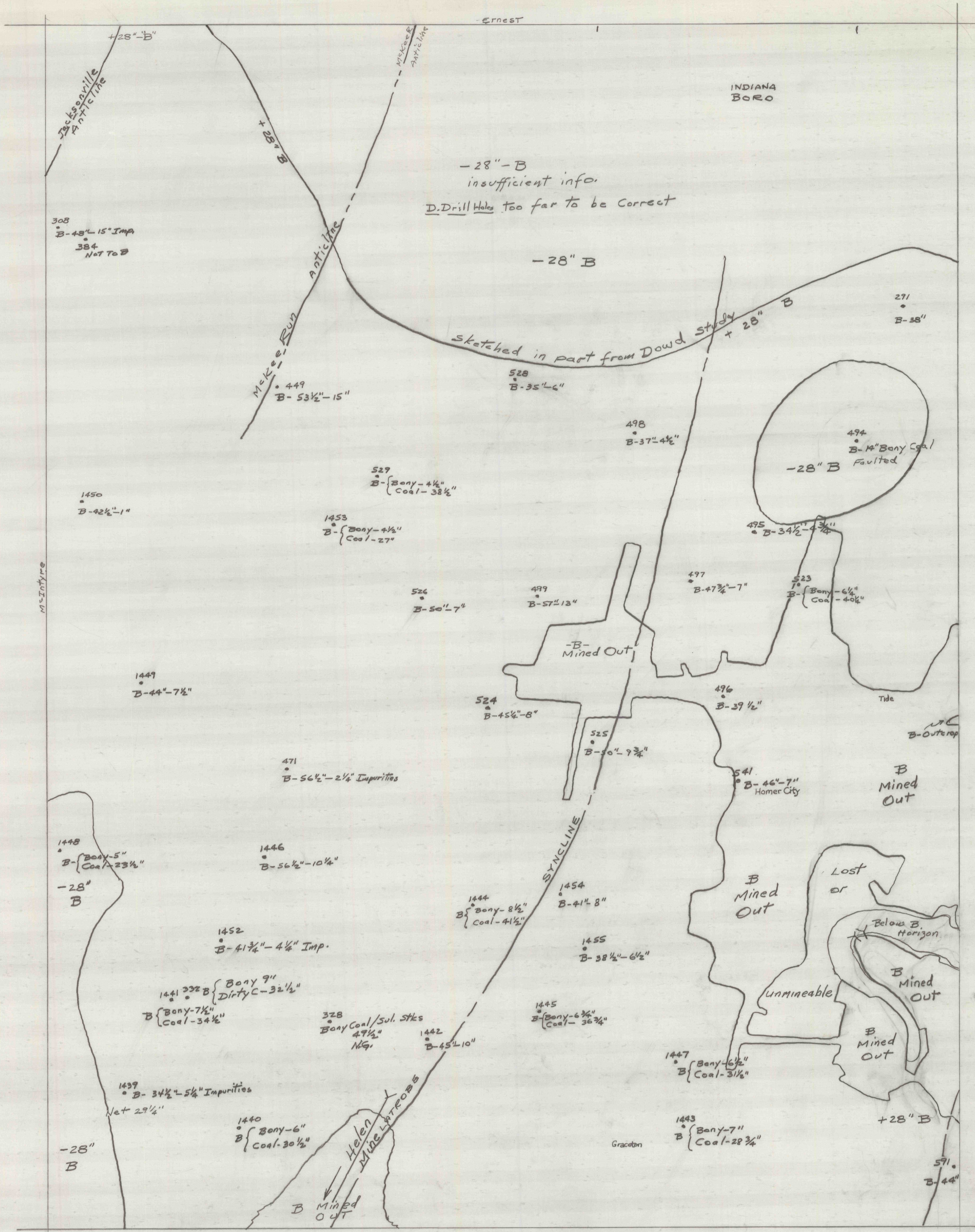
"B" SEAM-LOWER KITTANING INDIANA QUAD 1" = 2000'
