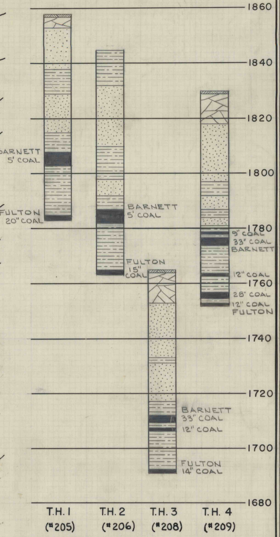
COLUMNAR SECTIONS SCALE: 1"=20'
