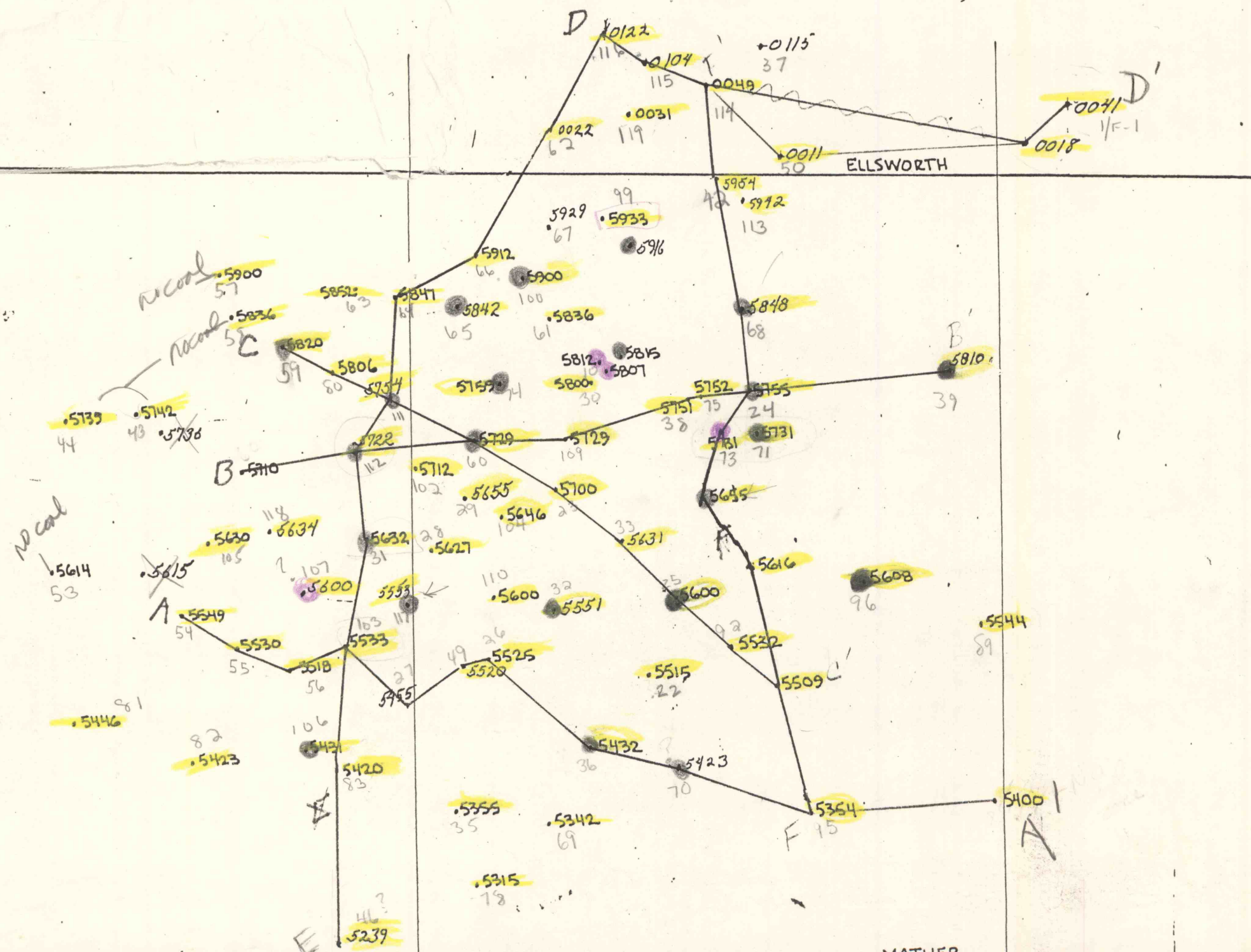
Fig. 15 Location map of Upper Freeport cross-sections
