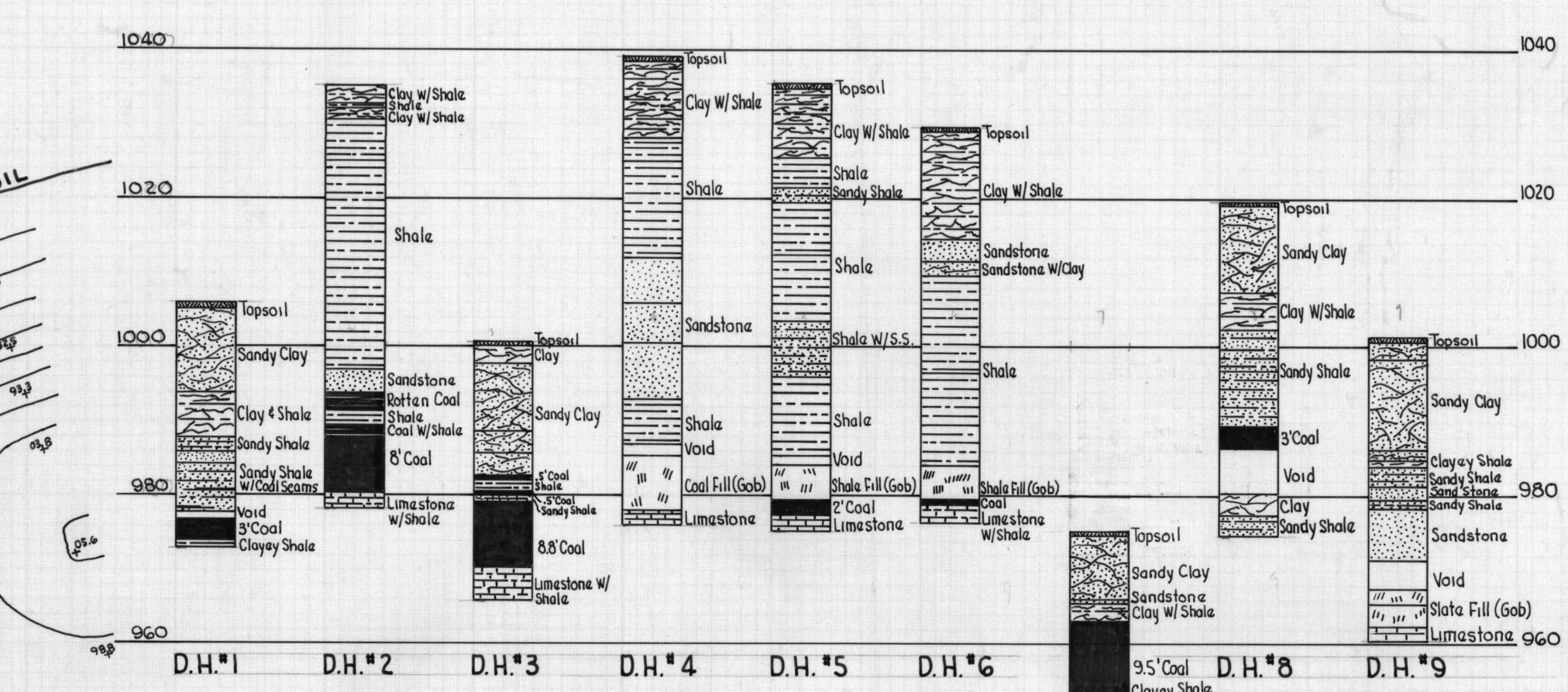
COLUMNAR SECTIONS SCALE: 1" = 20'
