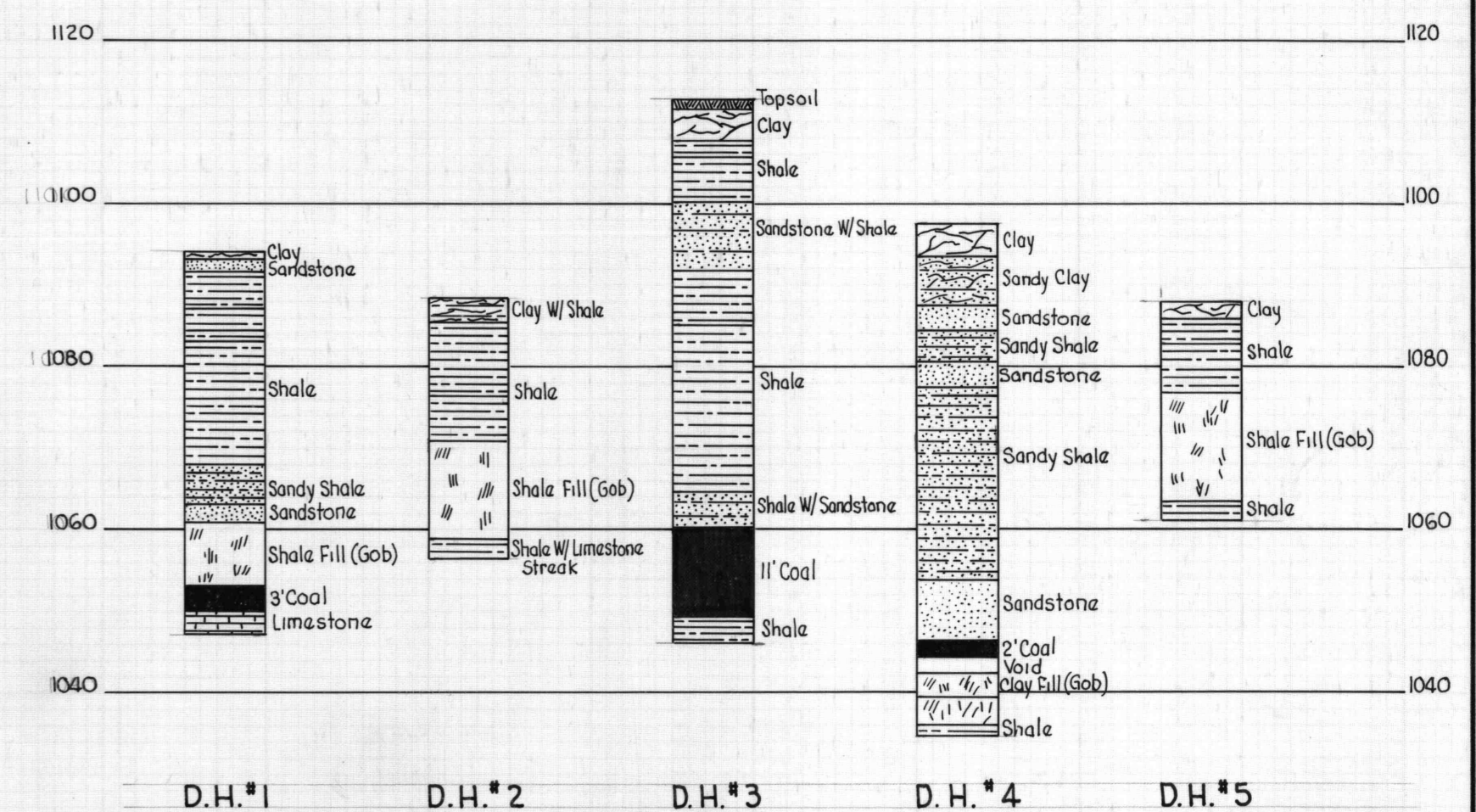
COLUMNAR SECTIONS
