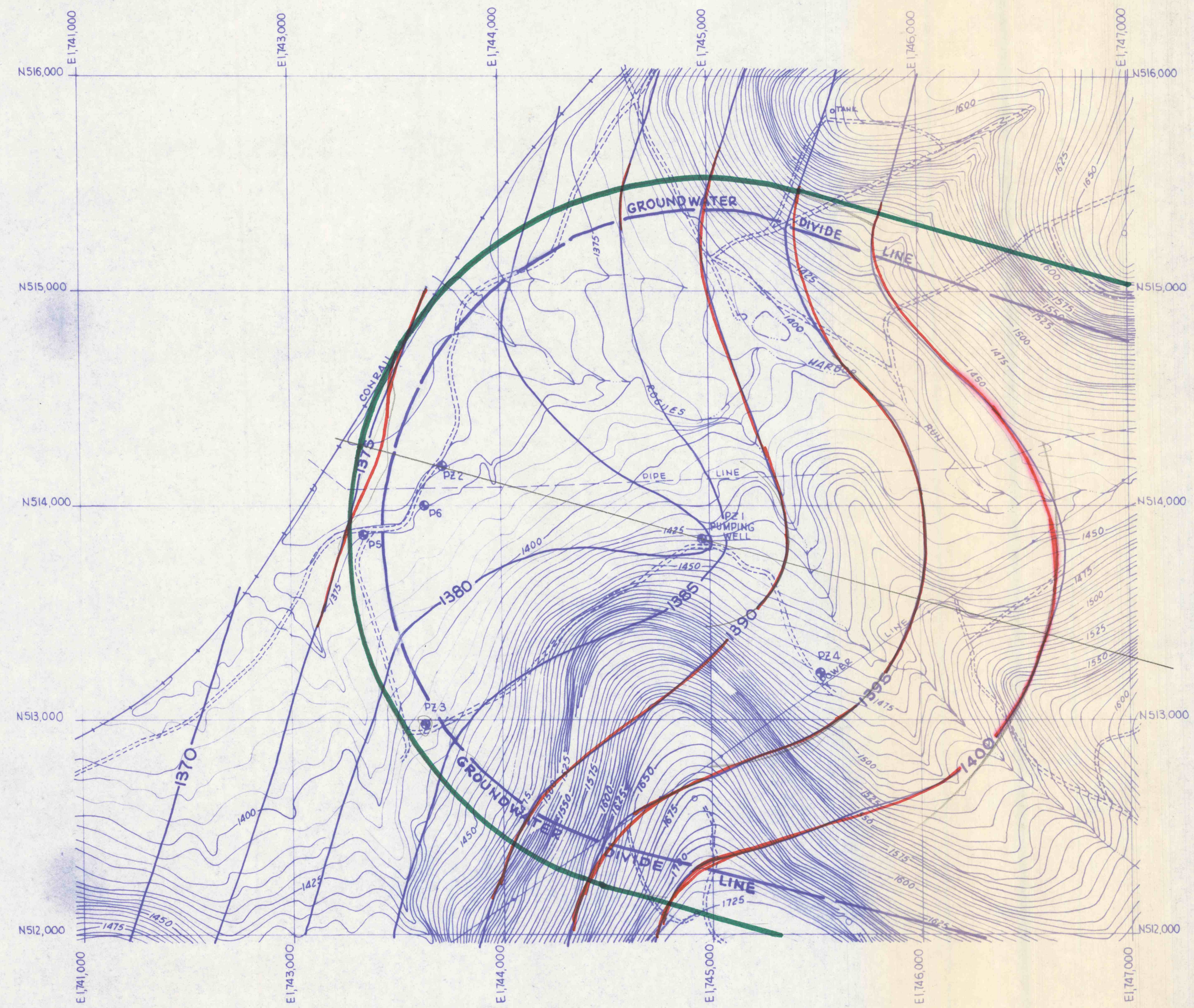
POST-PUMPING GROUND WATER CONTOURS SCALE: 1" = 400'
