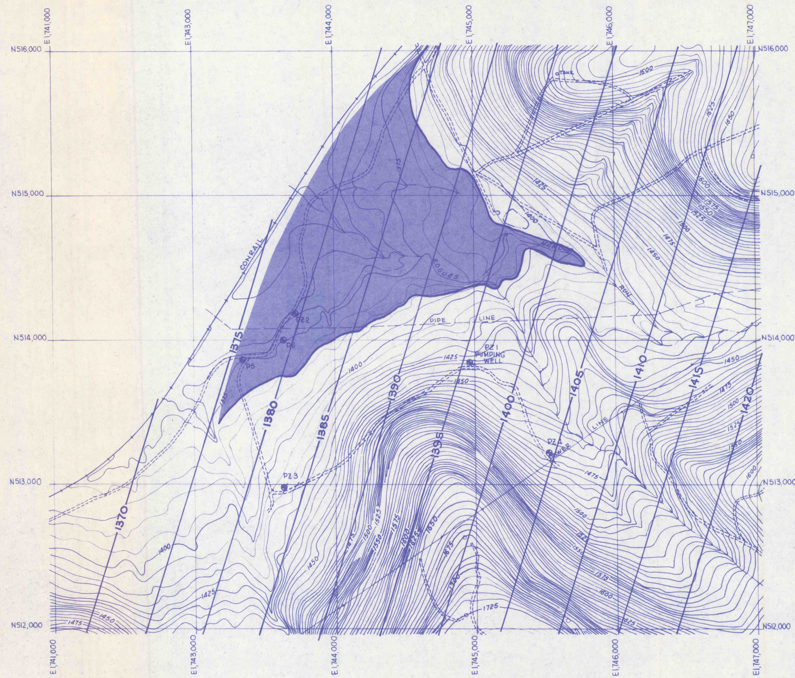
PRE-PUMPING GROUND WATER CONTOURS SCALE: 1" = 400'
