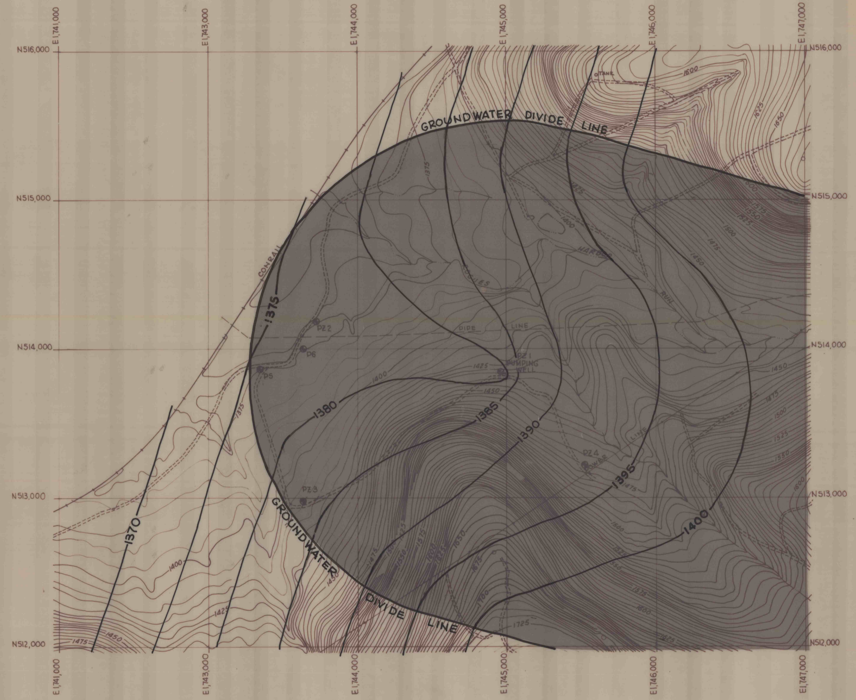
POST-PUMPING GROUND WATER CONTOURS
