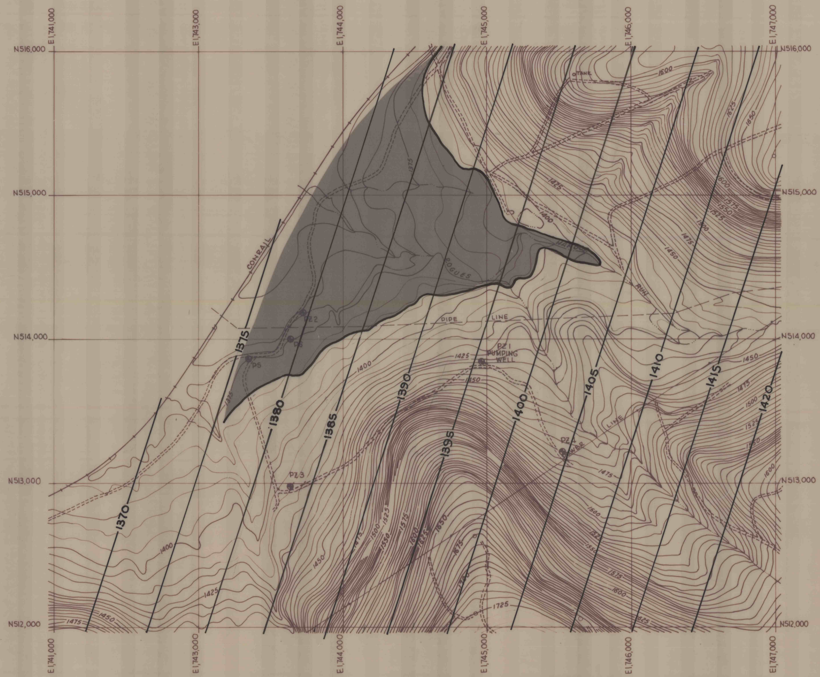
PRE-PUMPING GROUND WATER CONTOURS
