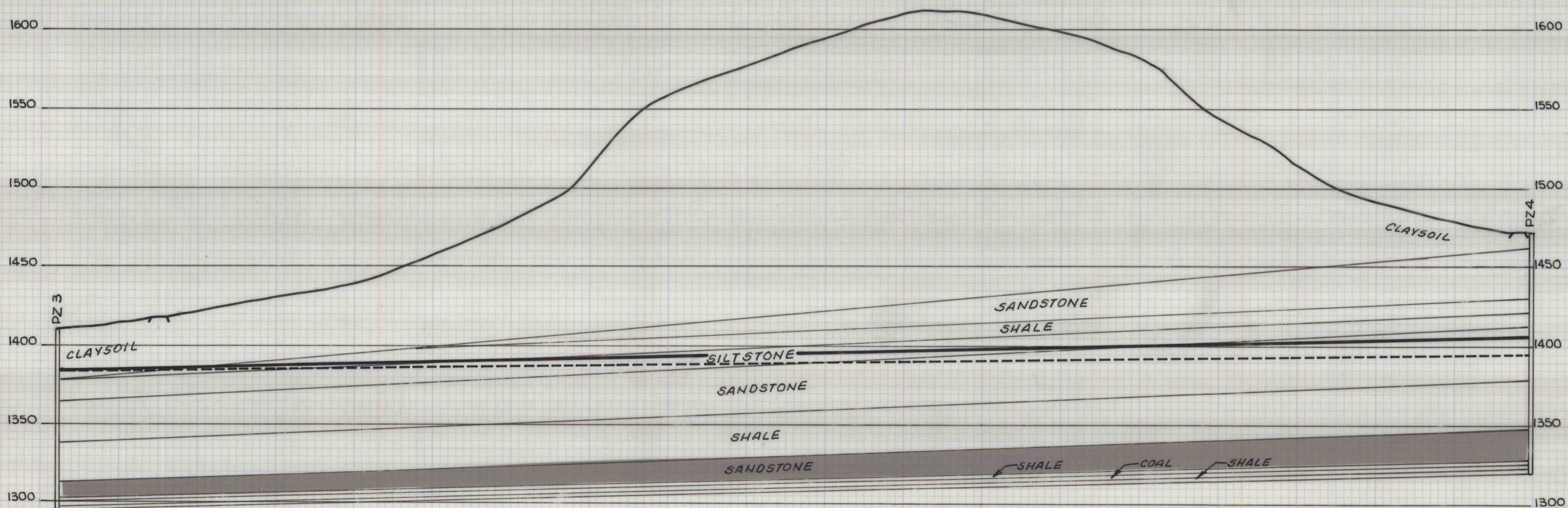
SECTION PZ 3 TO PZ 4
