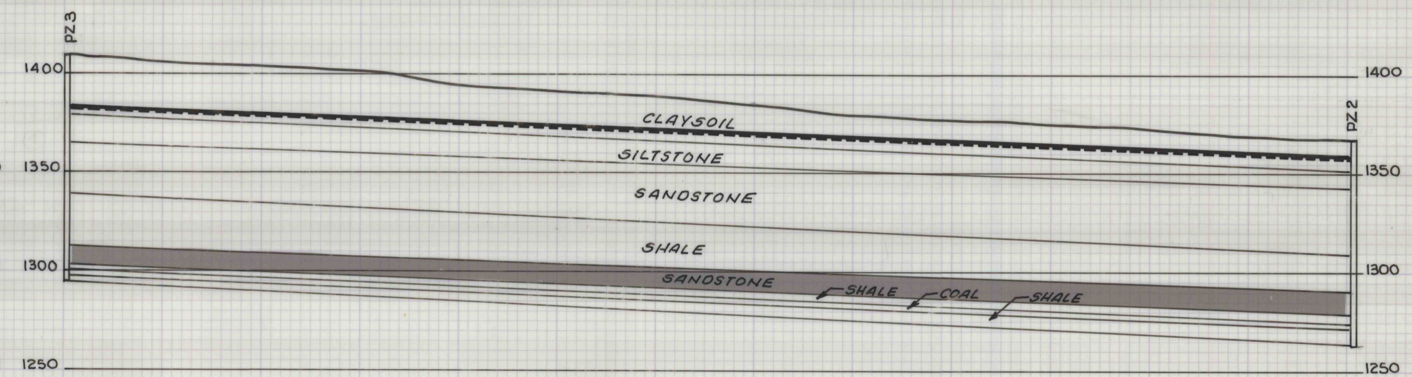
SECTION PZ 3 TO PZ 2
