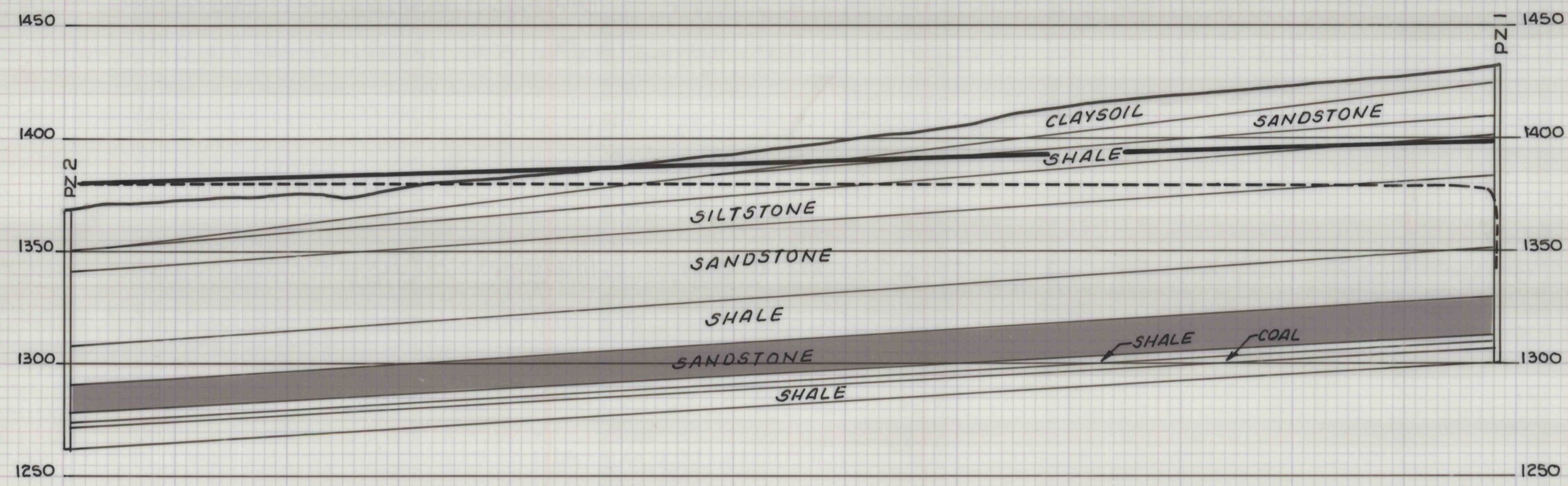
SECTION PZ 2 TO PZ 1
