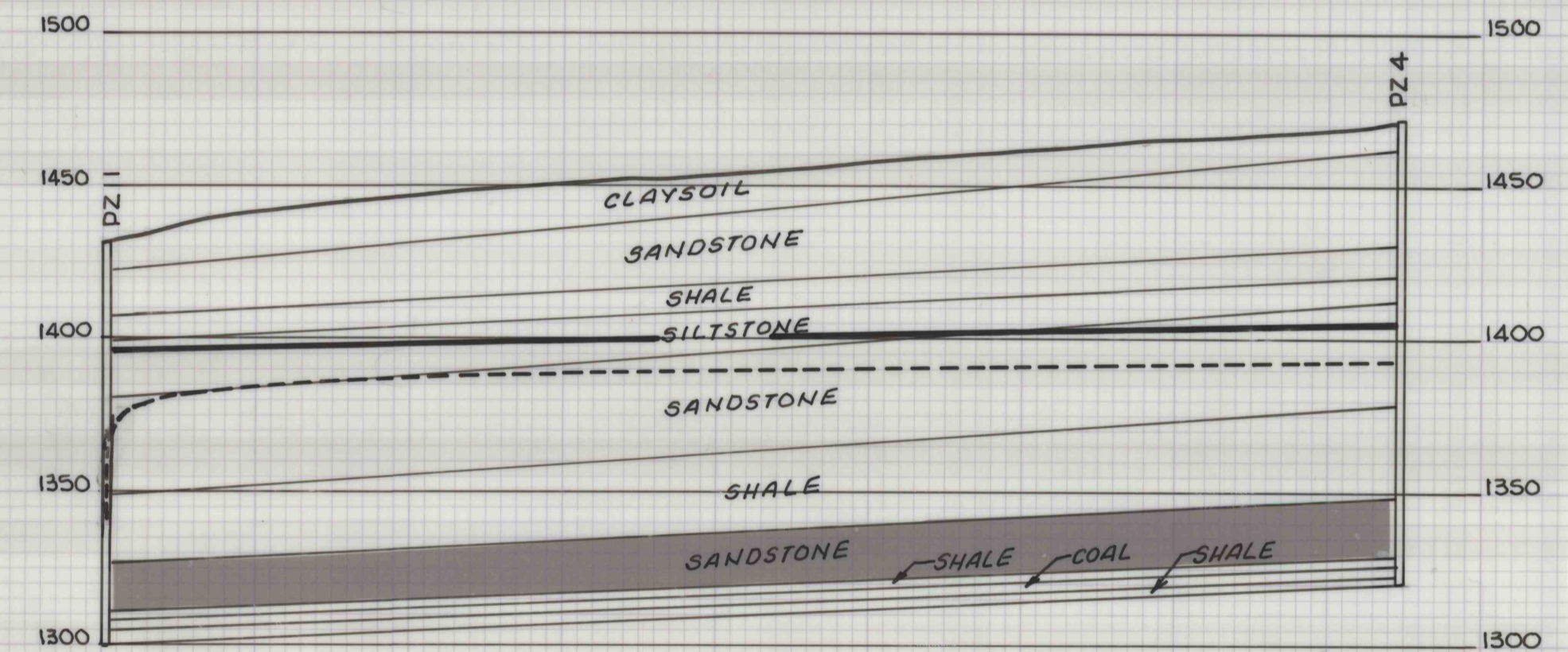
SECTION PZ 1 TO PZ 4
