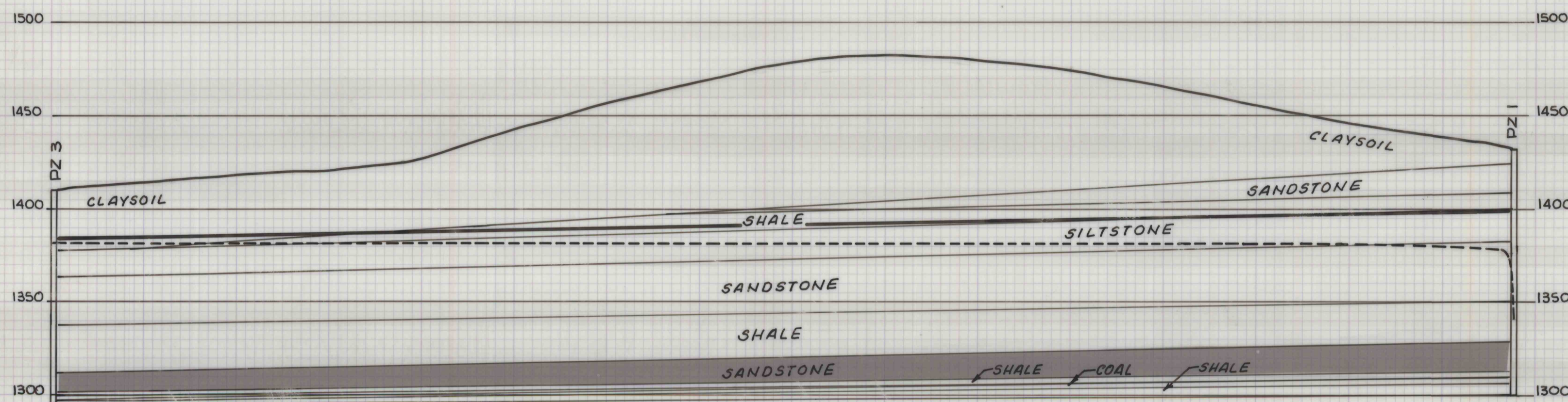
SECTION PZ 3 TO PZ 1
