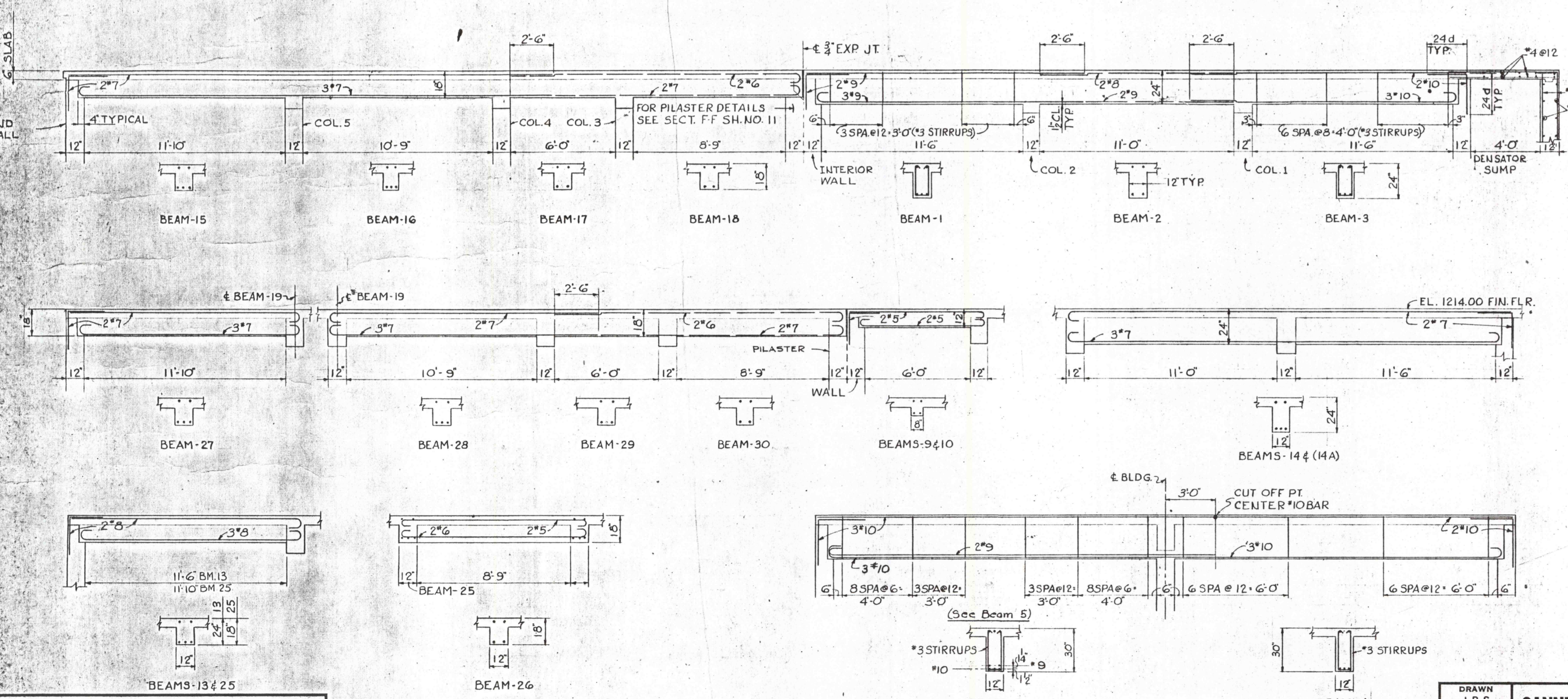
BEAM DETAILS
