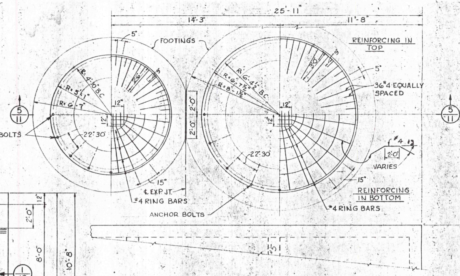
LIME STORAGE TANK FOUNDATION PLANS
