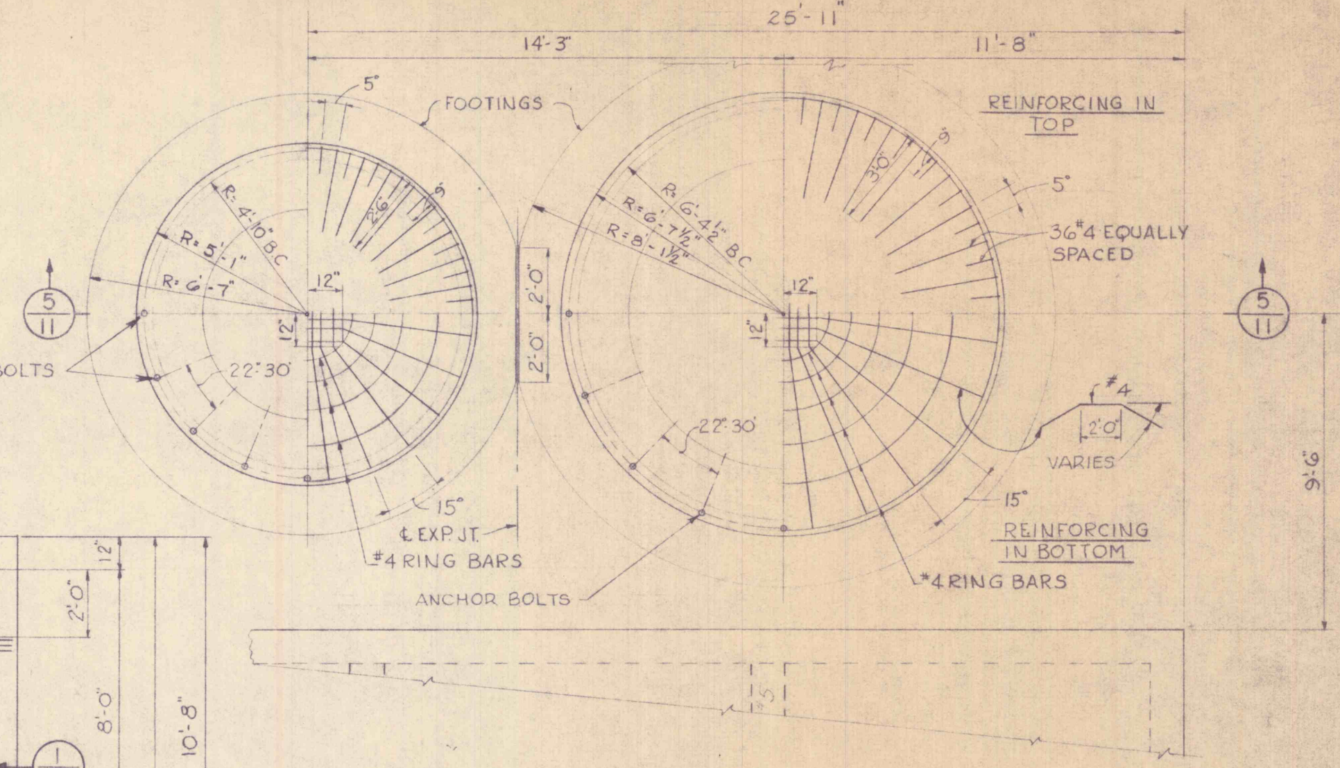
LIME STORAGE TANK FOUNDATION PLANS
