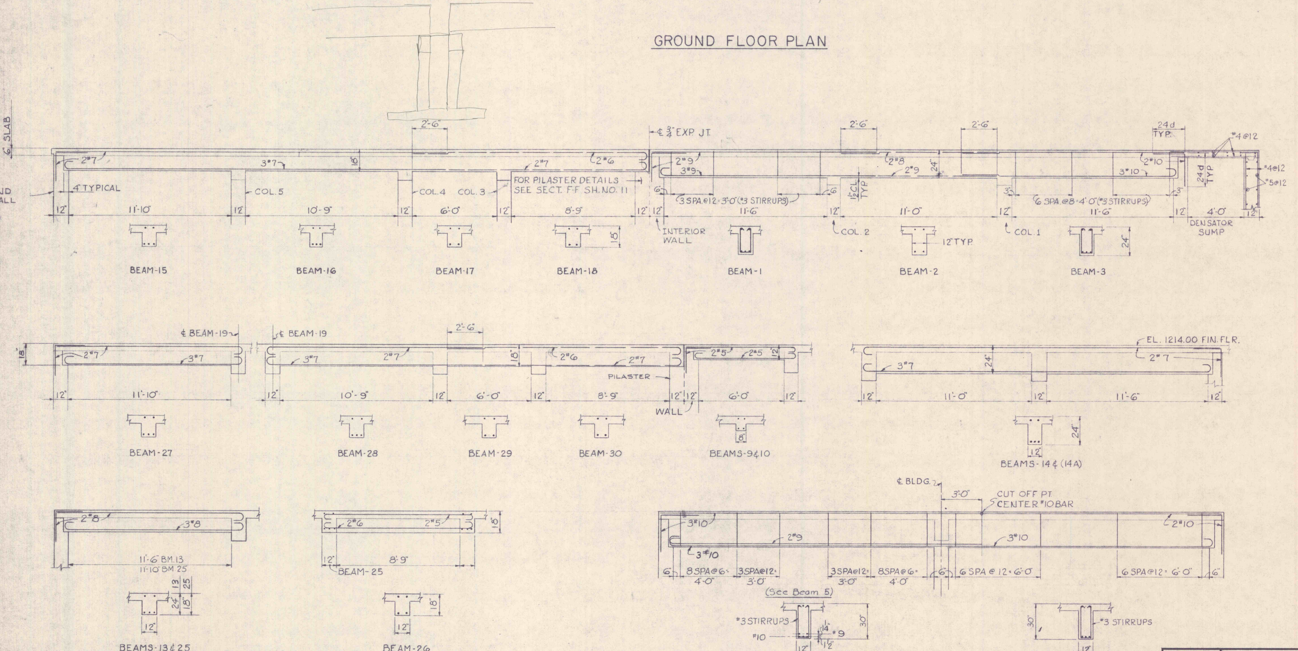
BEAM DETAILS
