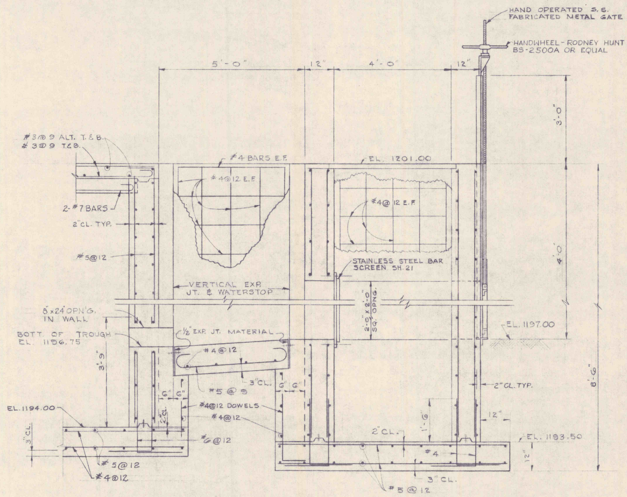
SECTION 1/17 SCALE 1/2"=1'-0"
