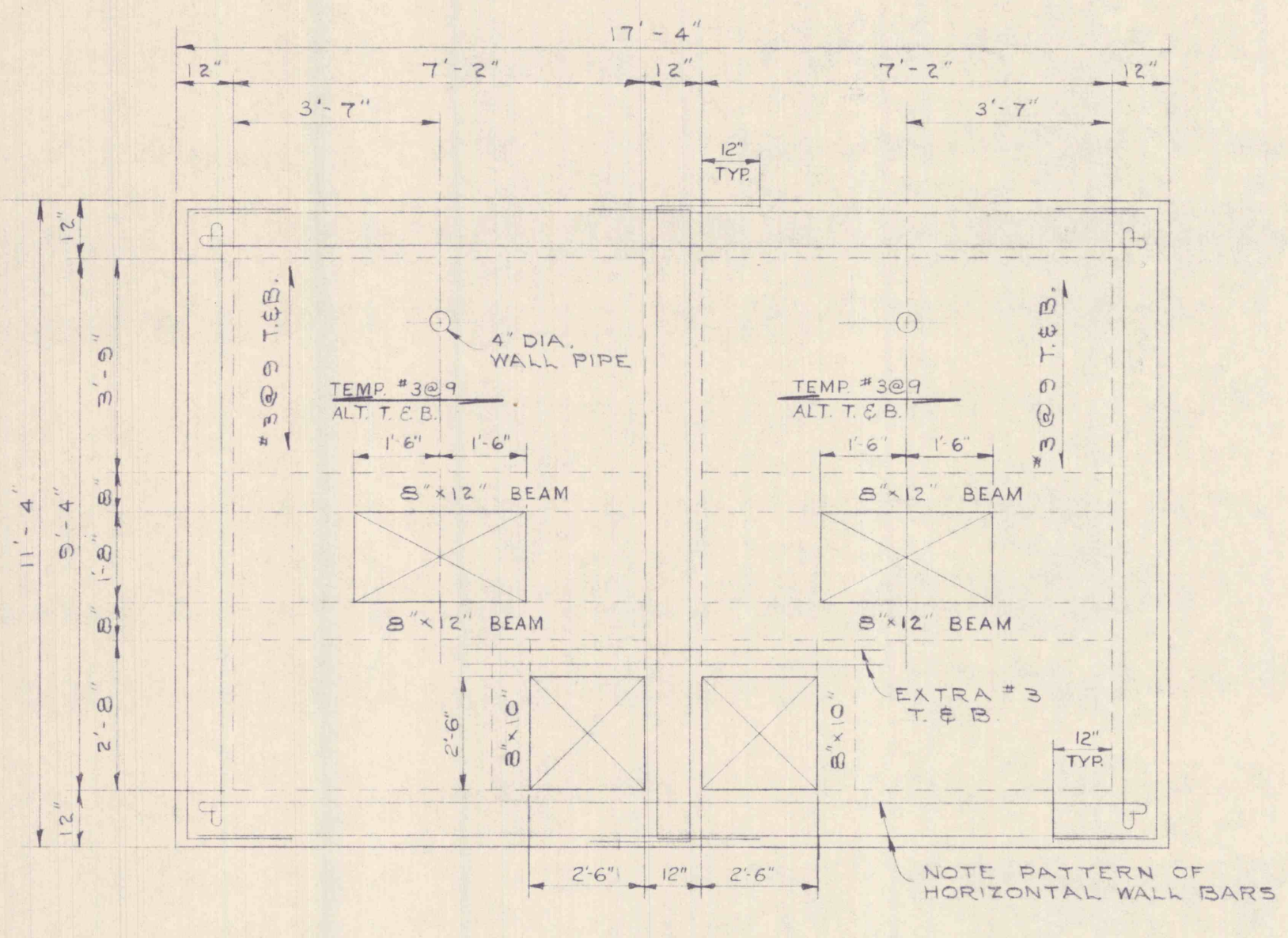
PUMPING STATION GROUND FLOOR PLAN STRUCTURAL SCALE 3/8"=1'-0"
