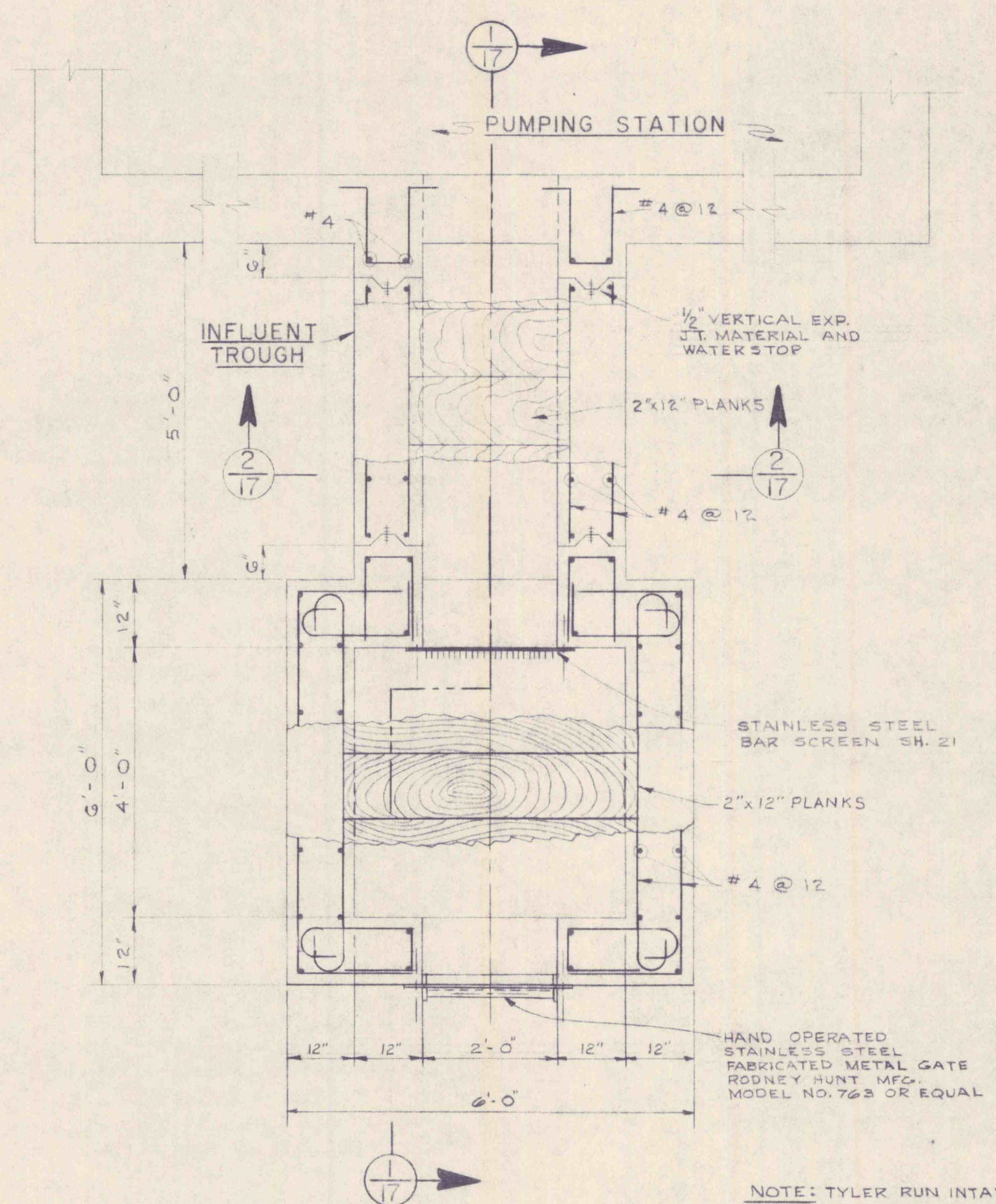
PLAN-PROCTOR NO. 2 INTAKE STRUCTURE SCALE 1/2"=1'-0"
