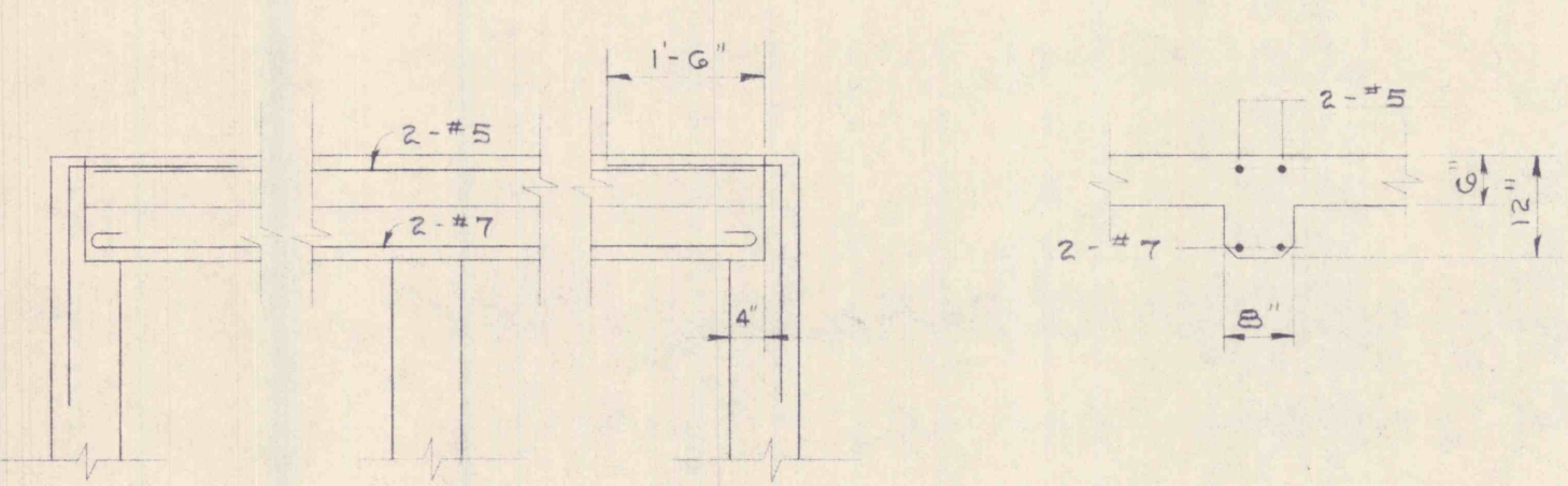
8" x 12" BEAM DETAILS NO SCALE
