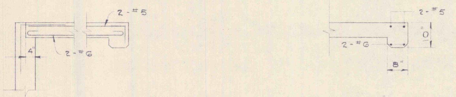
8" x 10" BEAM DETAILS NO SCALE
