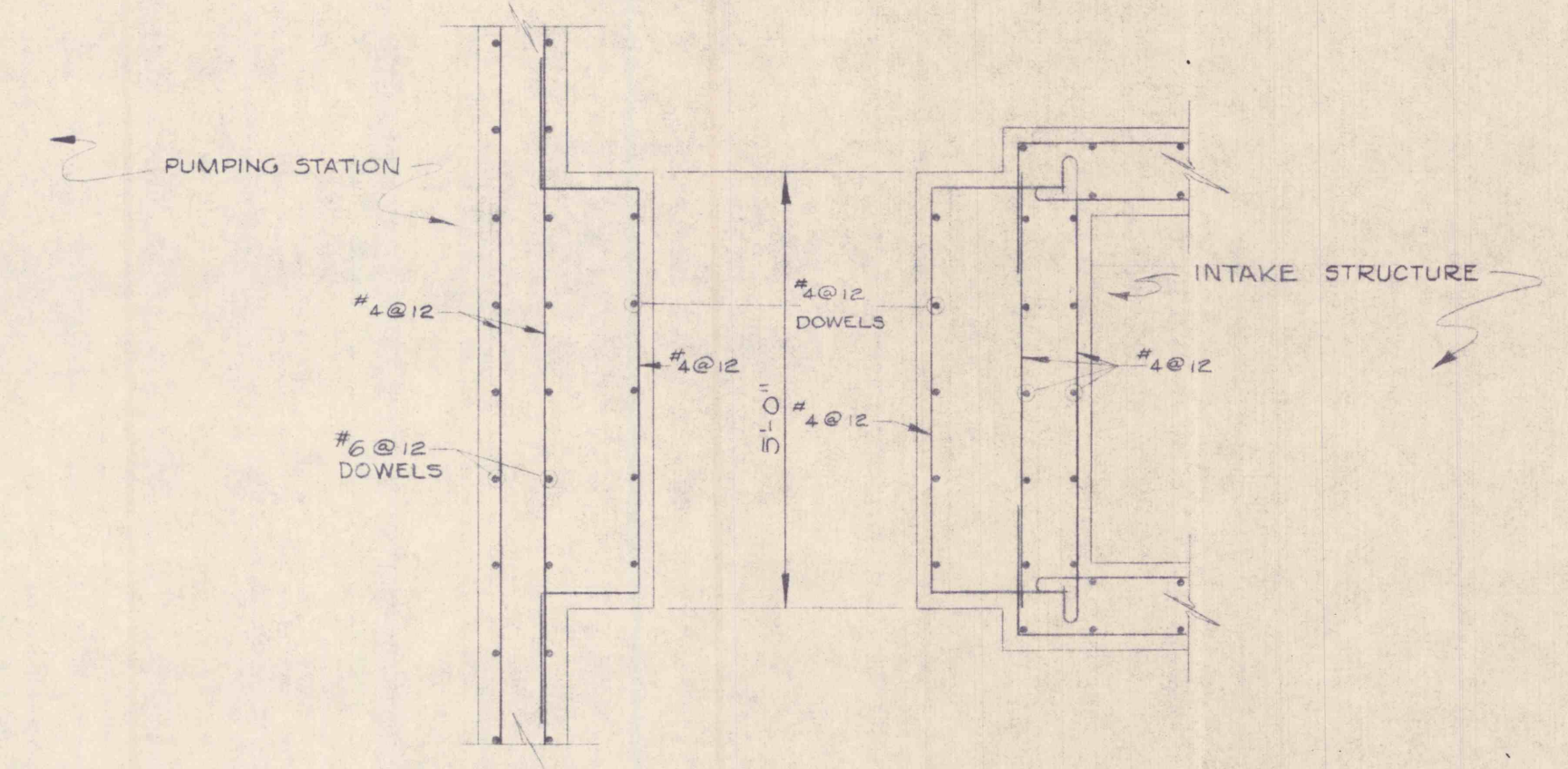
PLAN AT ELEV. 1195.0 SCALE 1/2"=1'-0"
