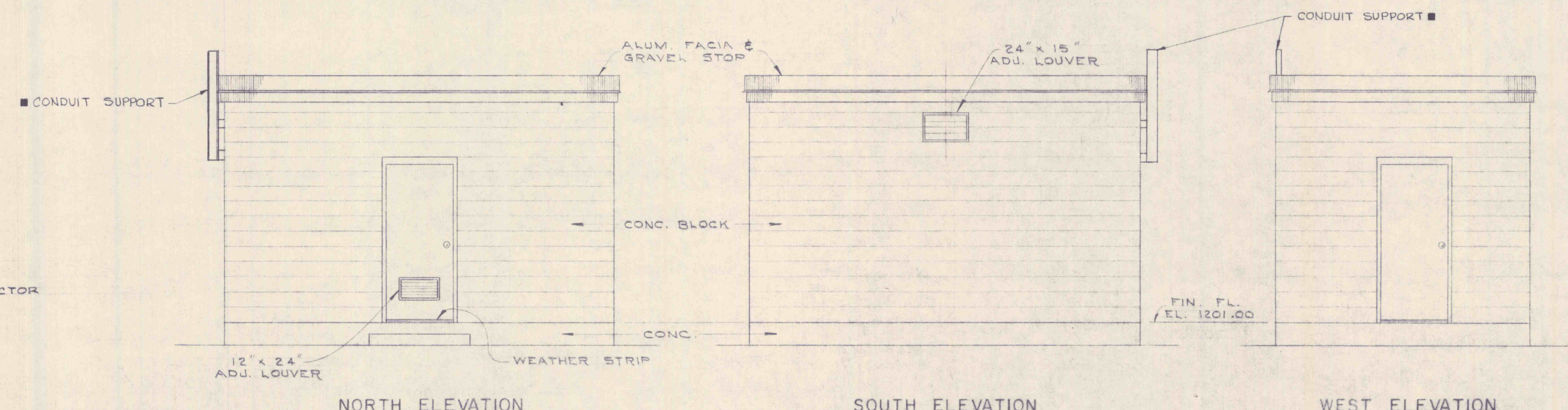
NORTH ELEVATION
