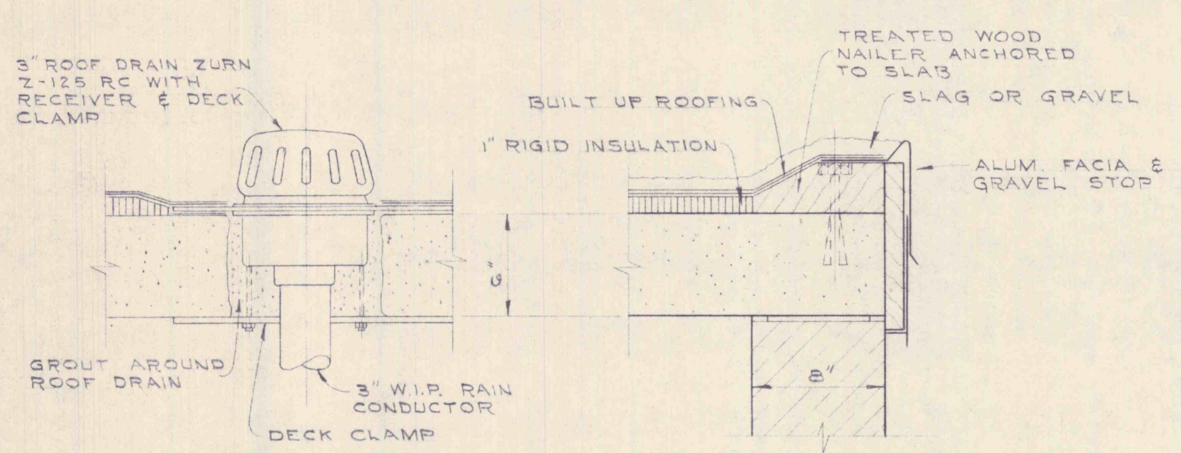
FACIA GRAVEL STOP & ROOF DRAIN DETAIL
