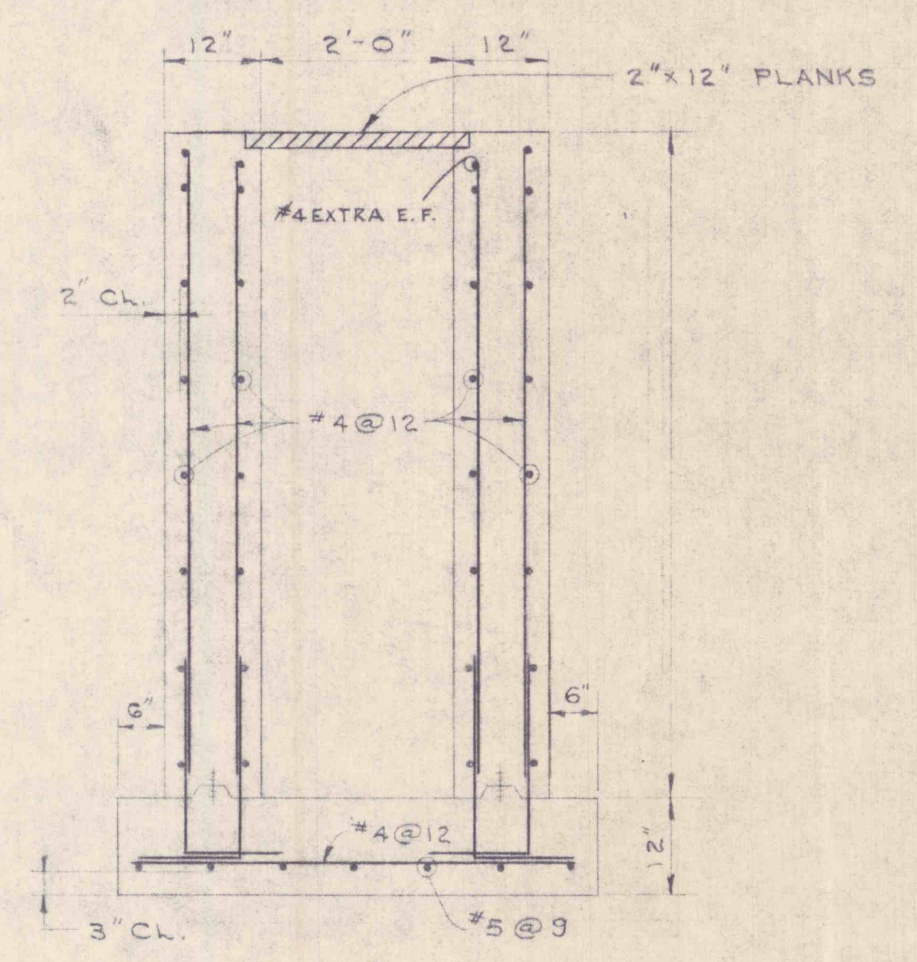
SECTION 2/17 SCALE 1/2"=1'-0"
