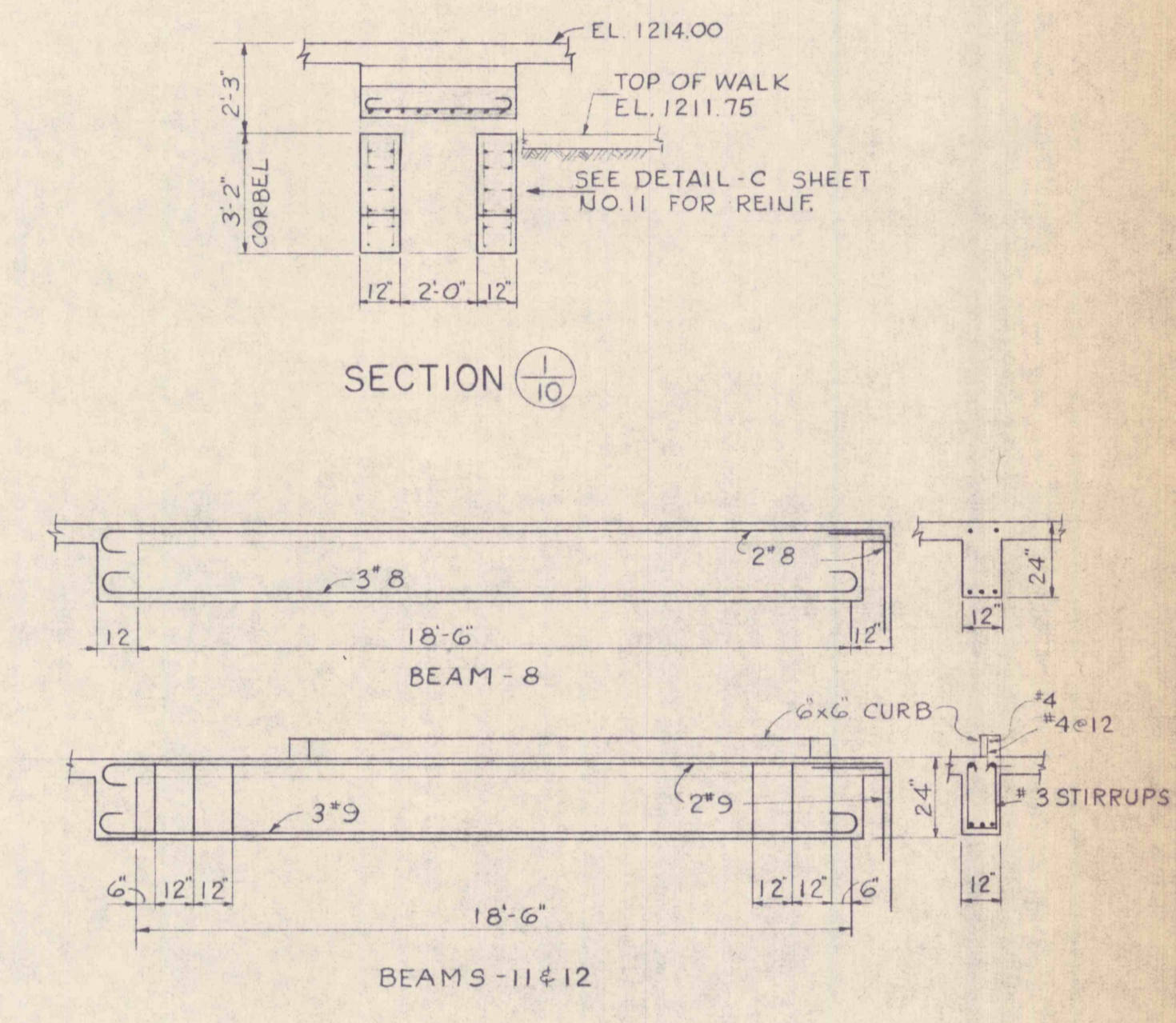
LIME STORAGE TANK FOUNDATION PLANS
