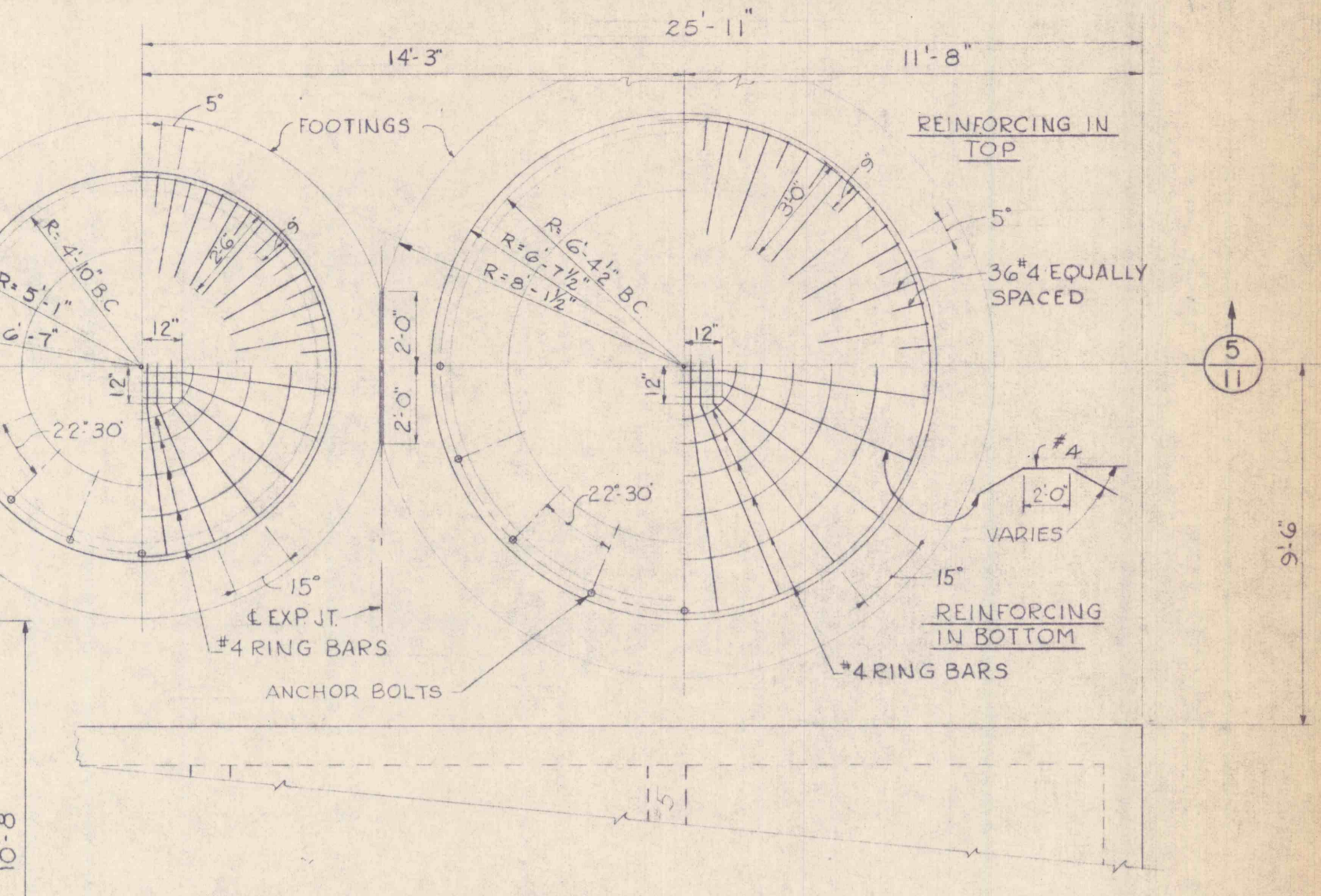
LIME STORAGE TANK FOUNDATION PLANS
