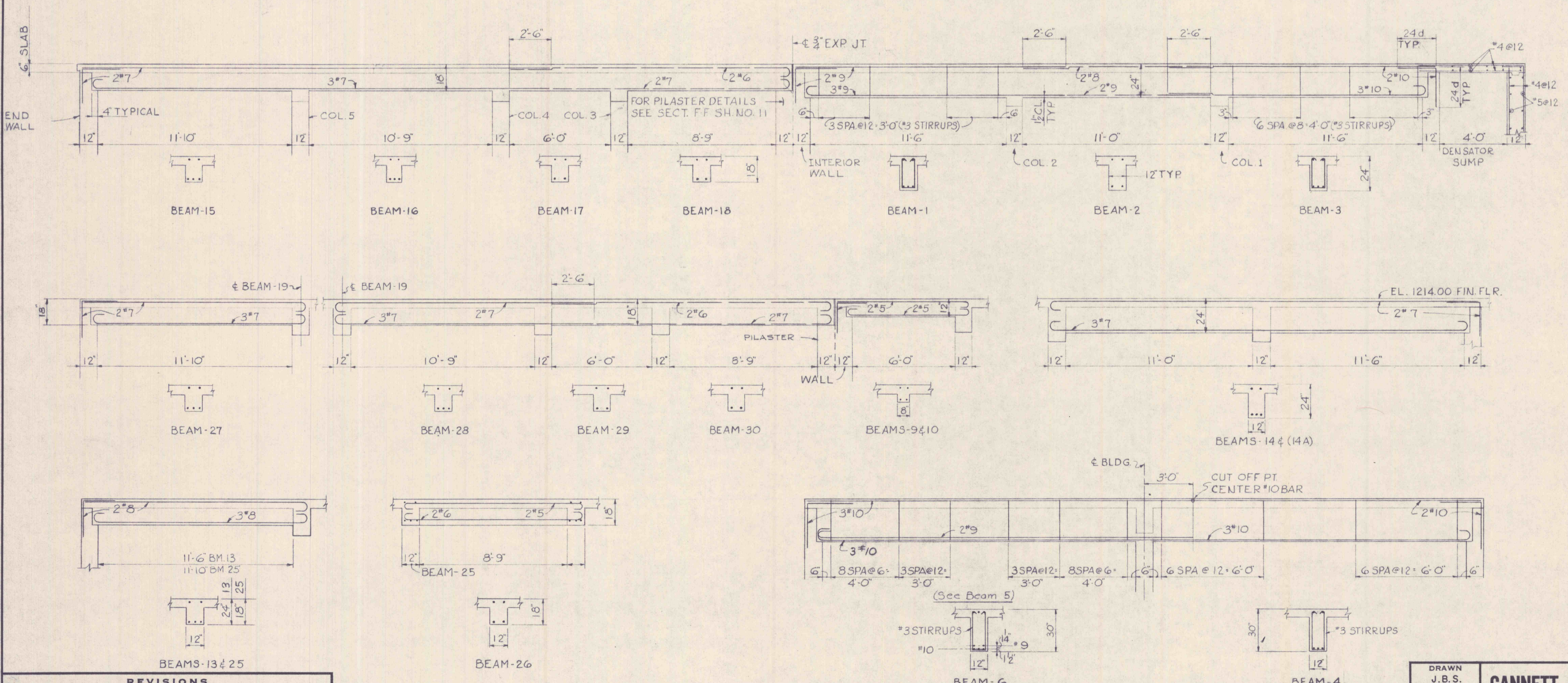
BEAM DETAILS
