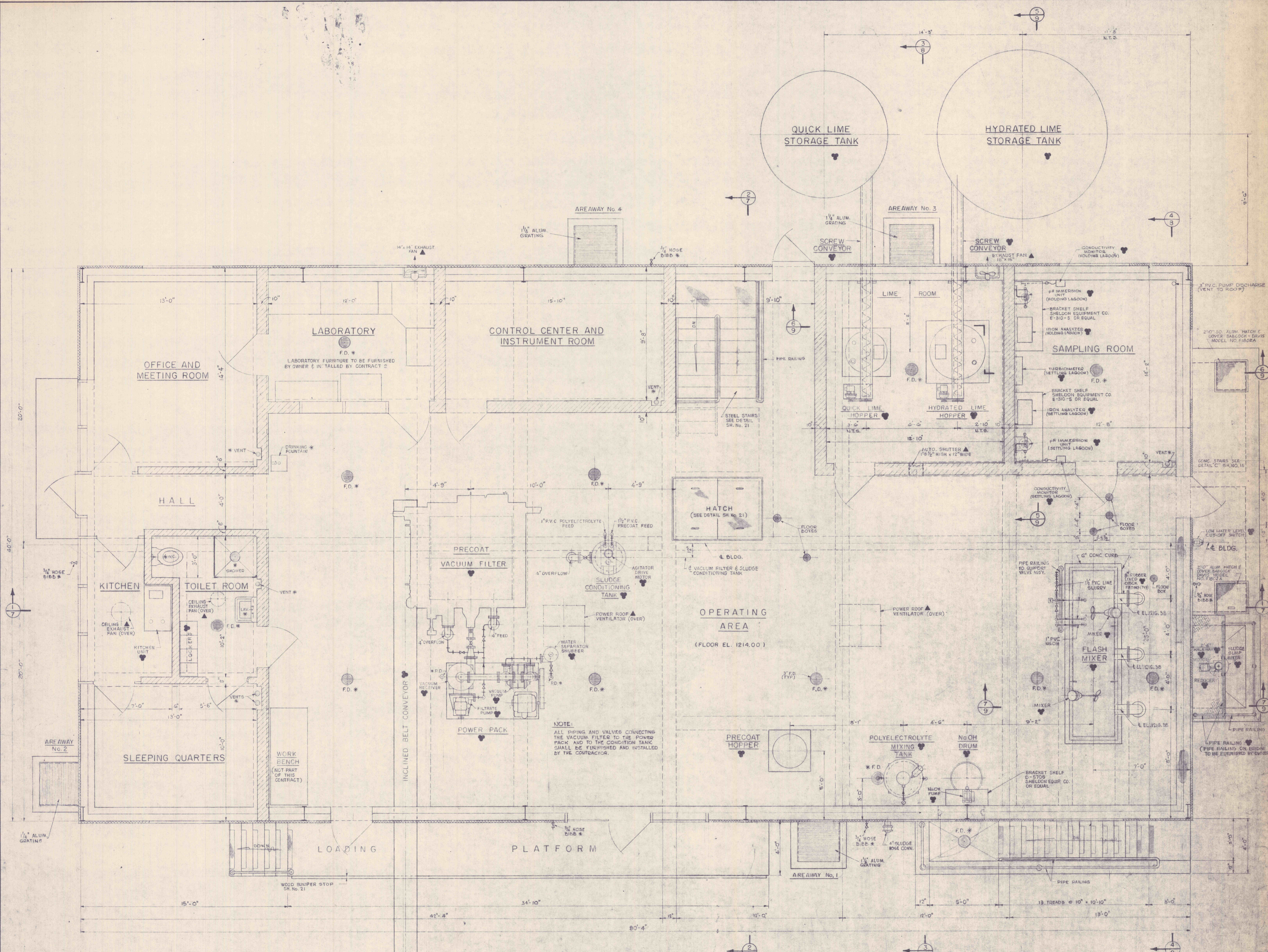
GROUND FLOOR PLAN SCALE 3/8" = 1'-0"
