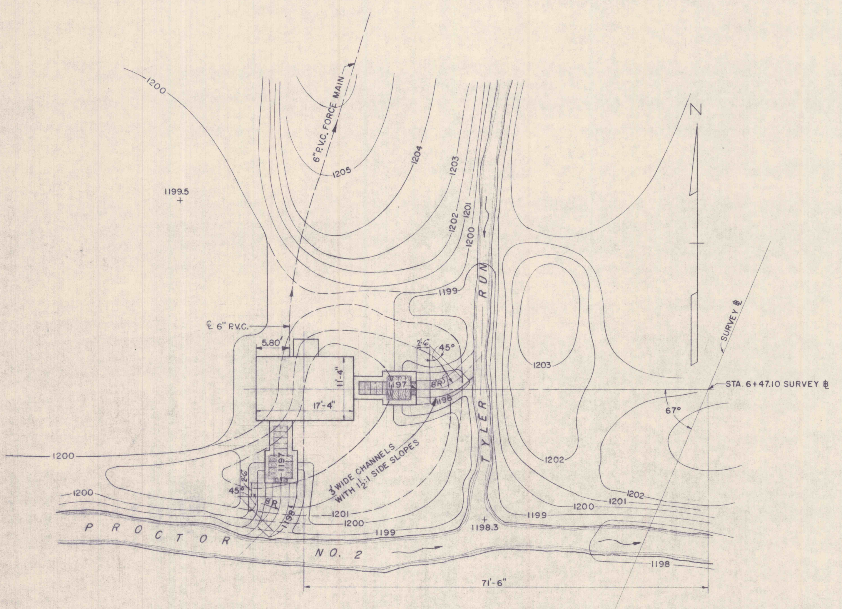
PROCTOR NO. 2 PUMPING STATION GRADING & LOCATION PLAN SCALE: 1" = 10'
