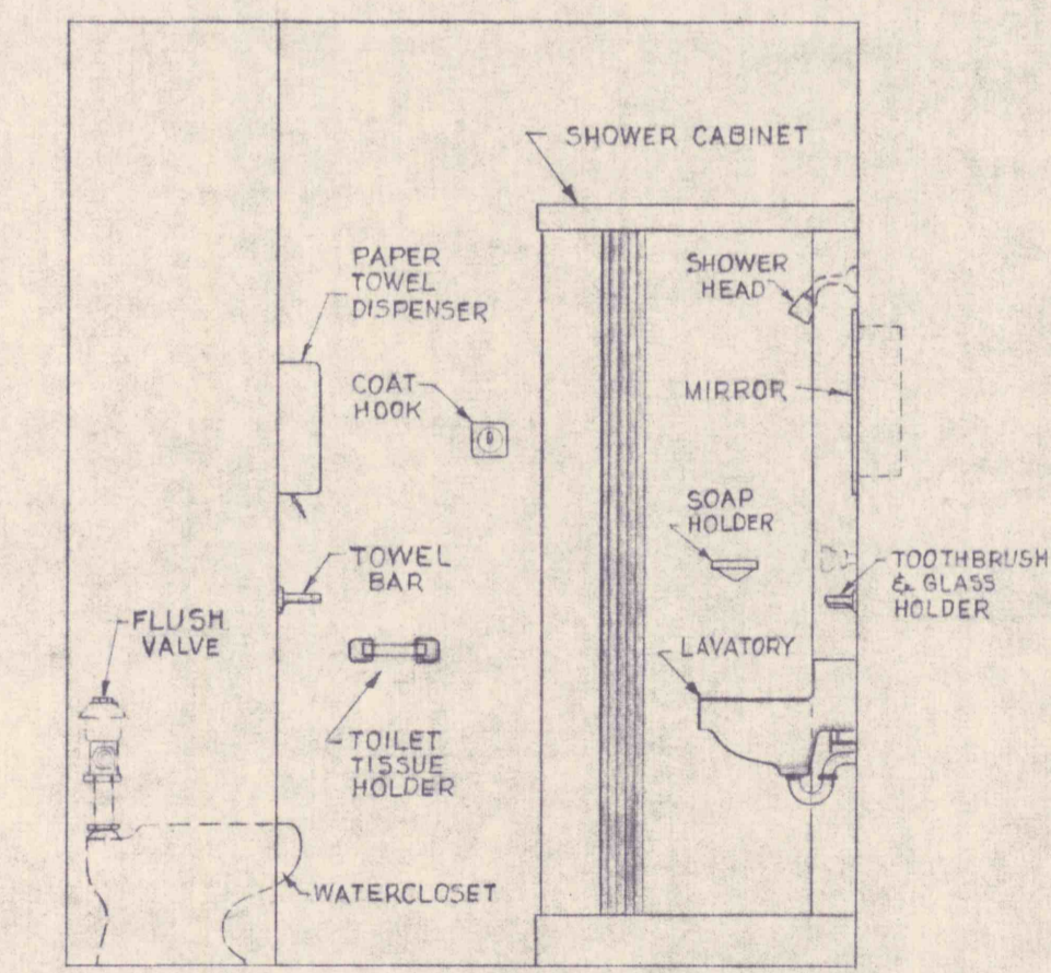
SECTION THRU TOILET RM. SCALE 1/2" = 1'-0"
