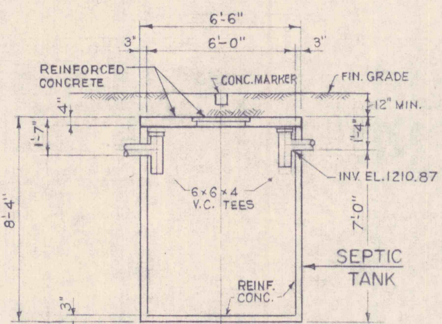
SECTION A-A SCALE 1/2" = 1'-0"
