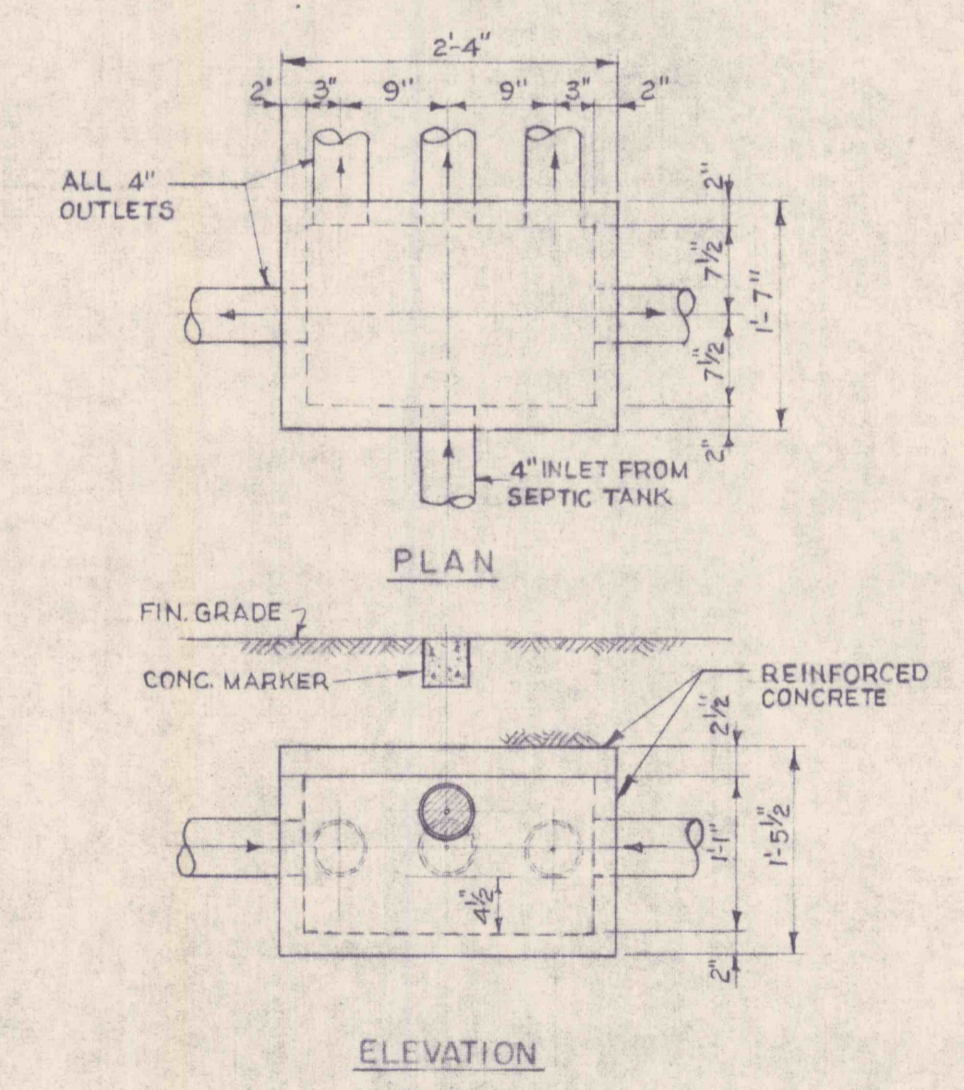
DISTRIBUTION BOX DETAIL SCALE 3/4" = 1'-0"
