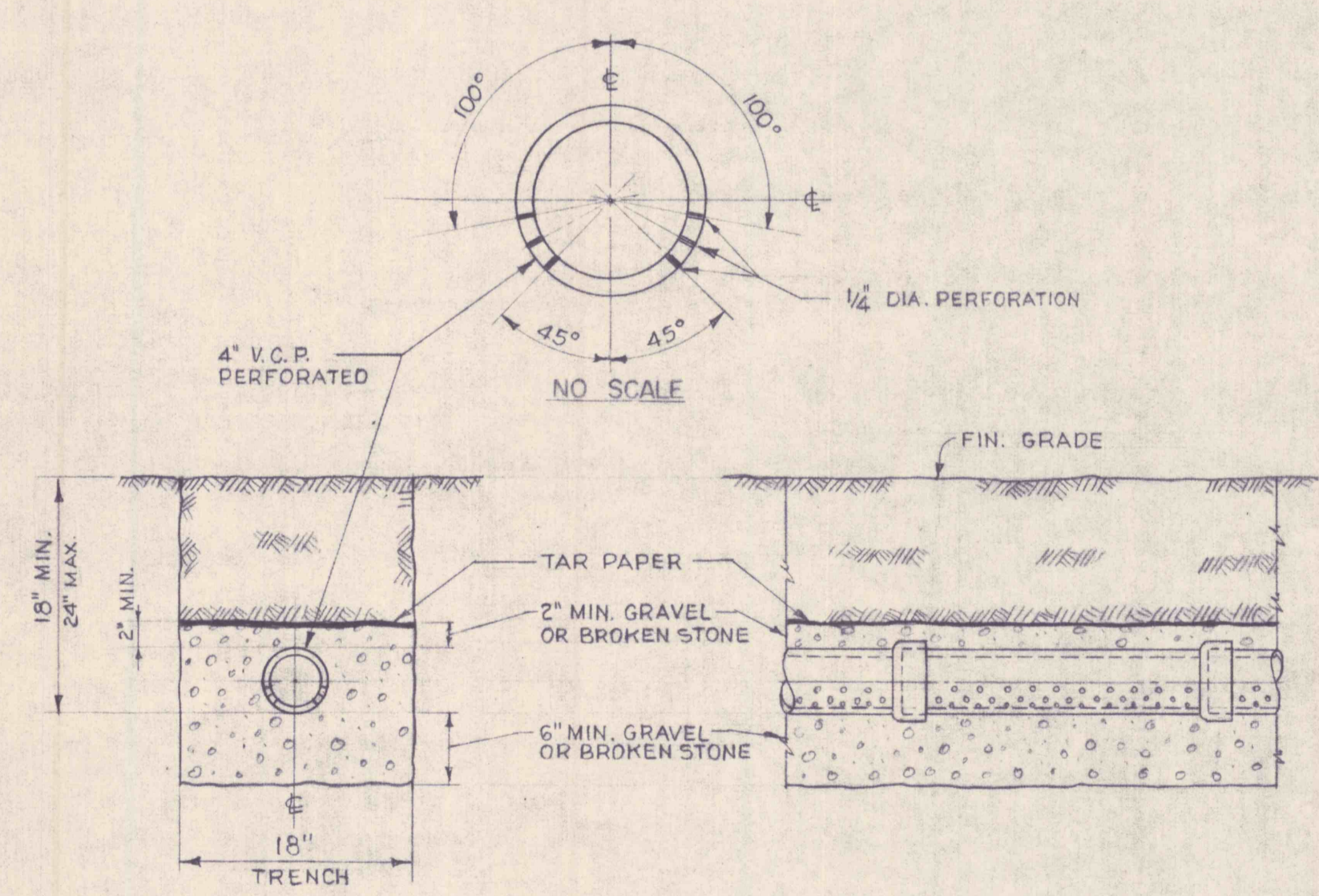
TILE FIELD TRENCH DETAILS SCALE 1" = 1'-0"
