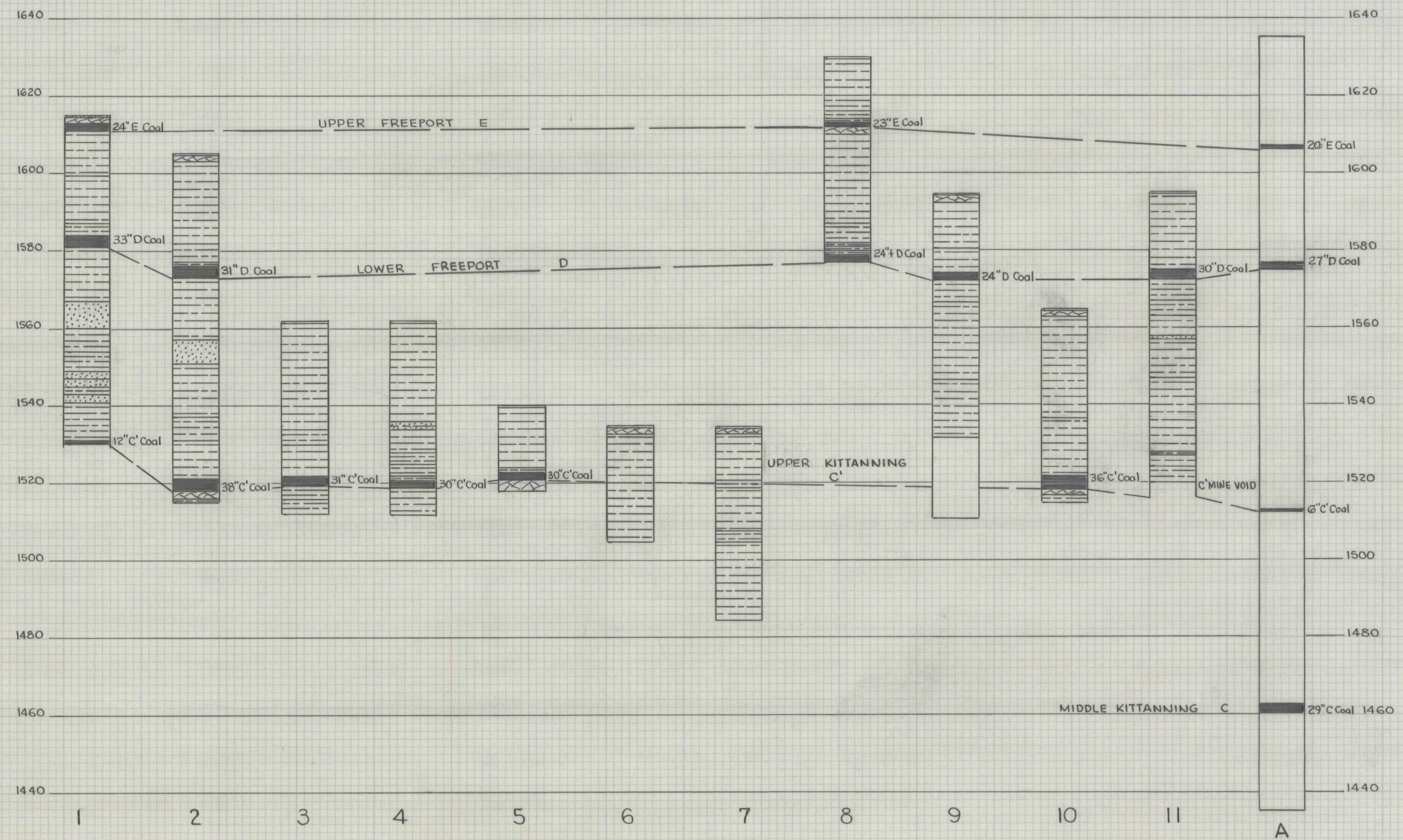
COLUMNAR SECTIONS SCALE: 1" = 20'
