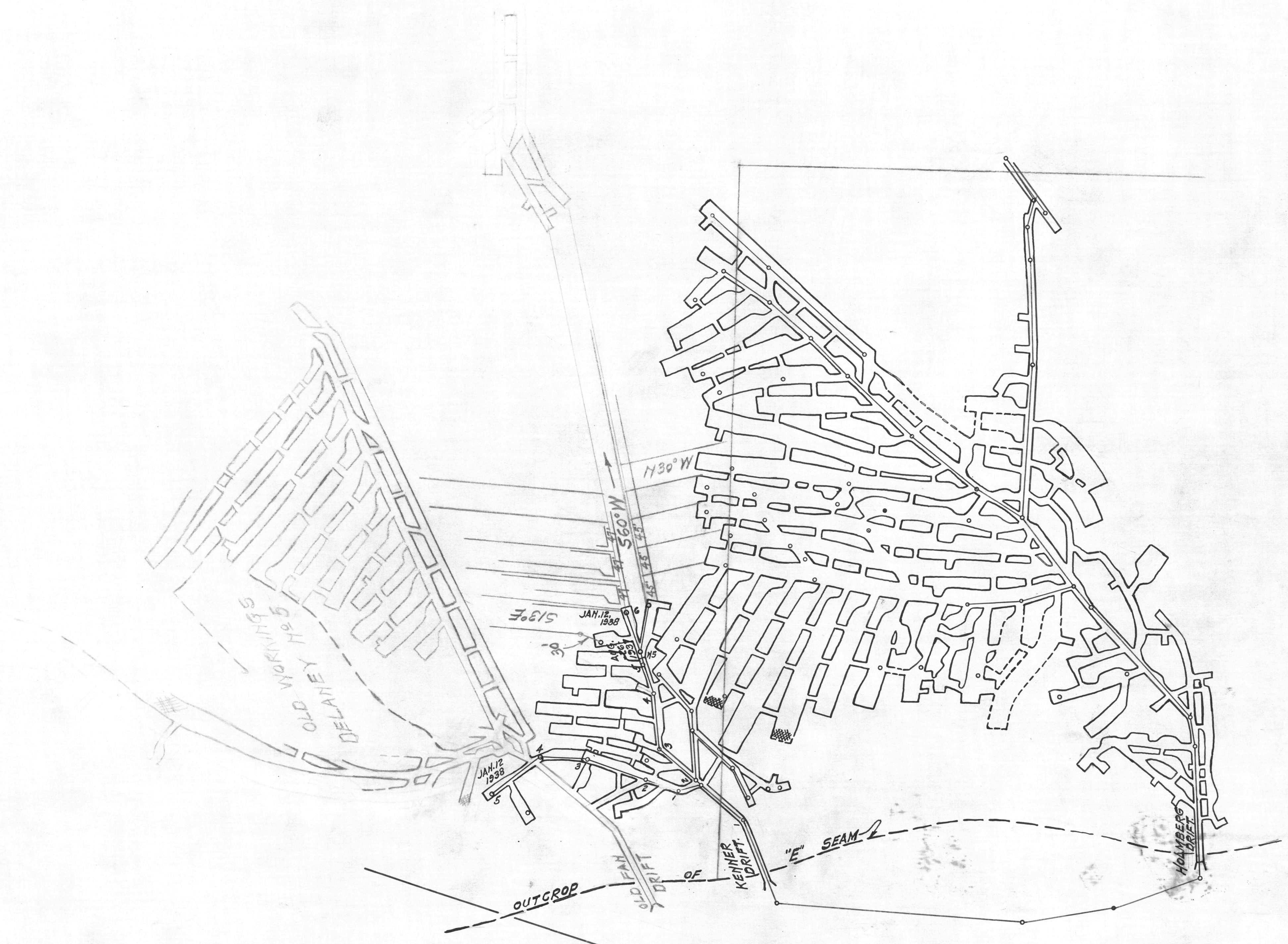
MINING OPERATIONS OF H. G. KENNER IN 'E' OR UPPER FREEPORT SEAM GALLITZIN TOWNSHIP, CAMBRIA COUNTY, PA. SCALE: - 1" = 100' SILLIMAN & WESTLEY MINING ENGRS. ALTOONA, PA.
