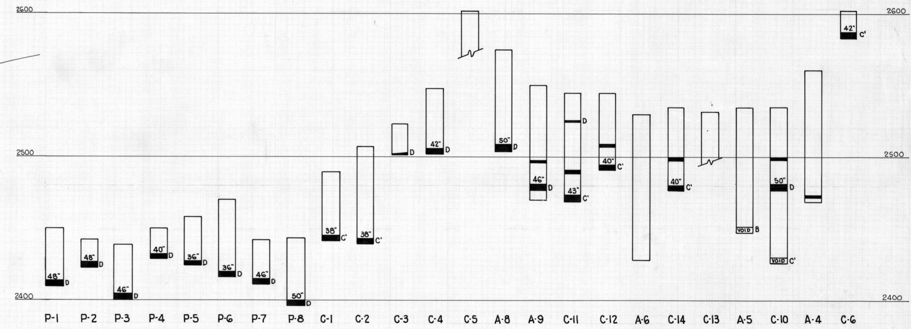
COLUMNAR SECTIONS OF DRILL HOLES
