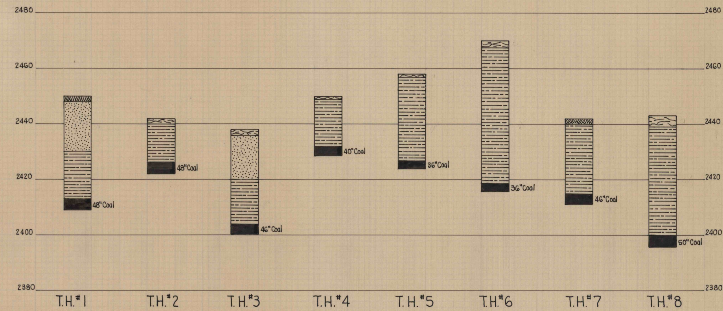
COLUMNAR SECTIONS OF TEST HOLES SCALE: 1" = 20'
