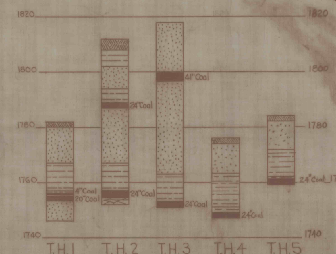
COLUMNAR SECTIONS SCALE: 1" = 20'
