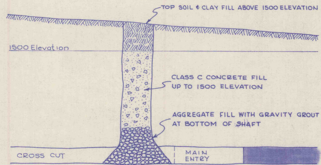
SKETCH SHOWING SECTION VIEW OF AIR SHAFT DETAILS SCALE: 1" = 10' Approx.
