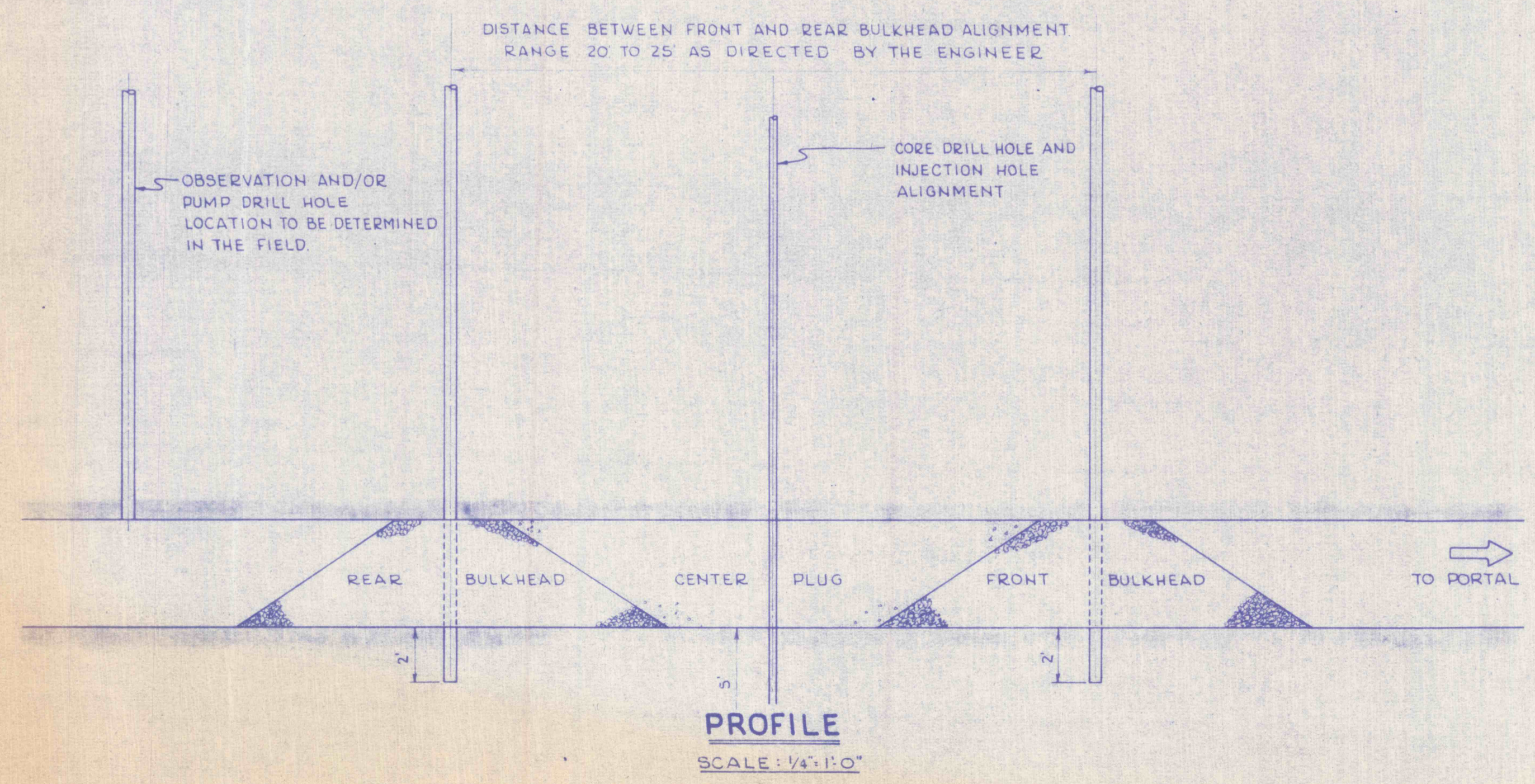
CONSTRUCTION DRAWING OF DEEP MINE SEAL
