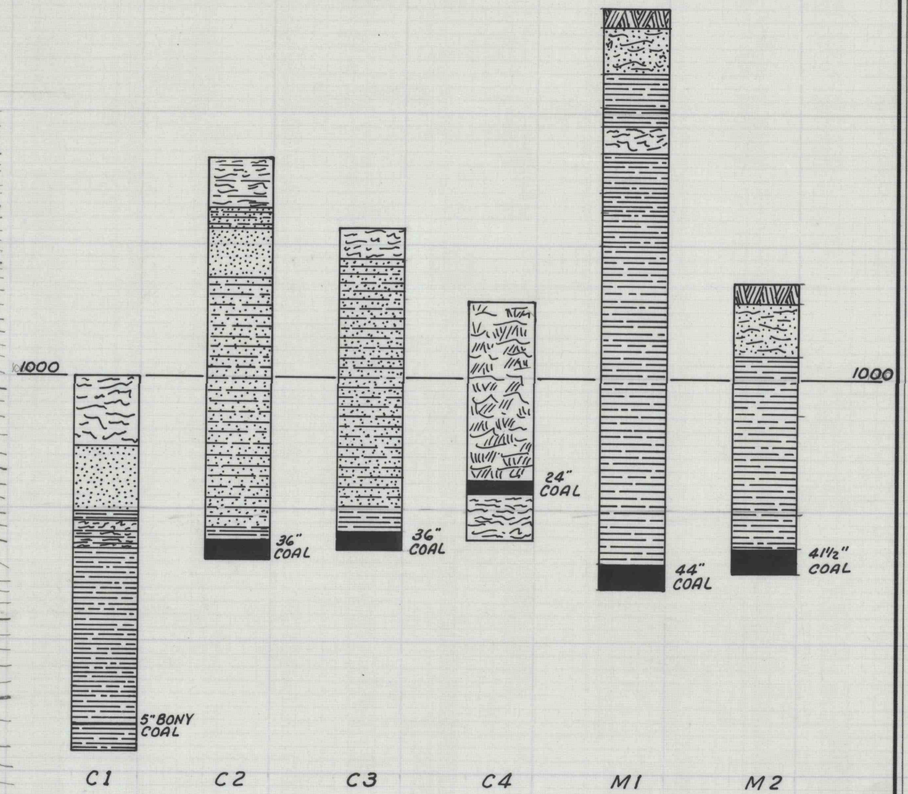
COLUMNAR SECTIONS OF DRILL HOLES SCALE: 1"=20'
