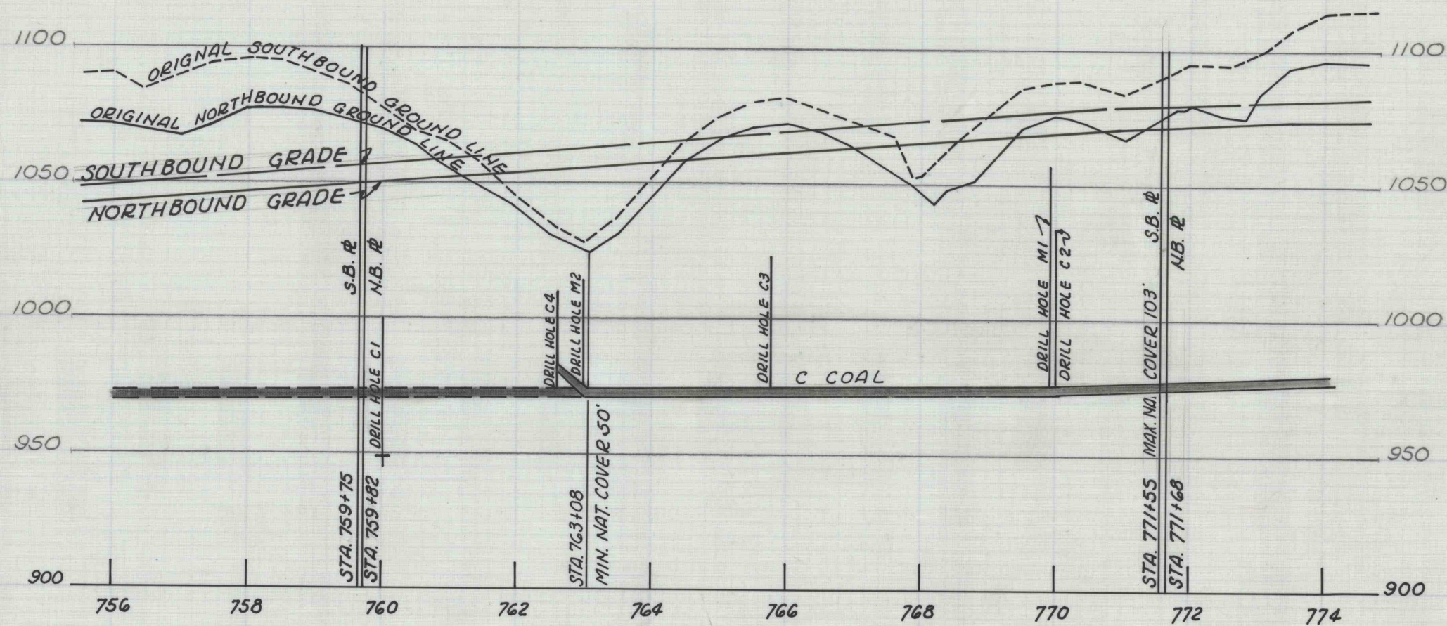
PROFILE 1"=200' HOR. SCALE: 1"=50' VER.
