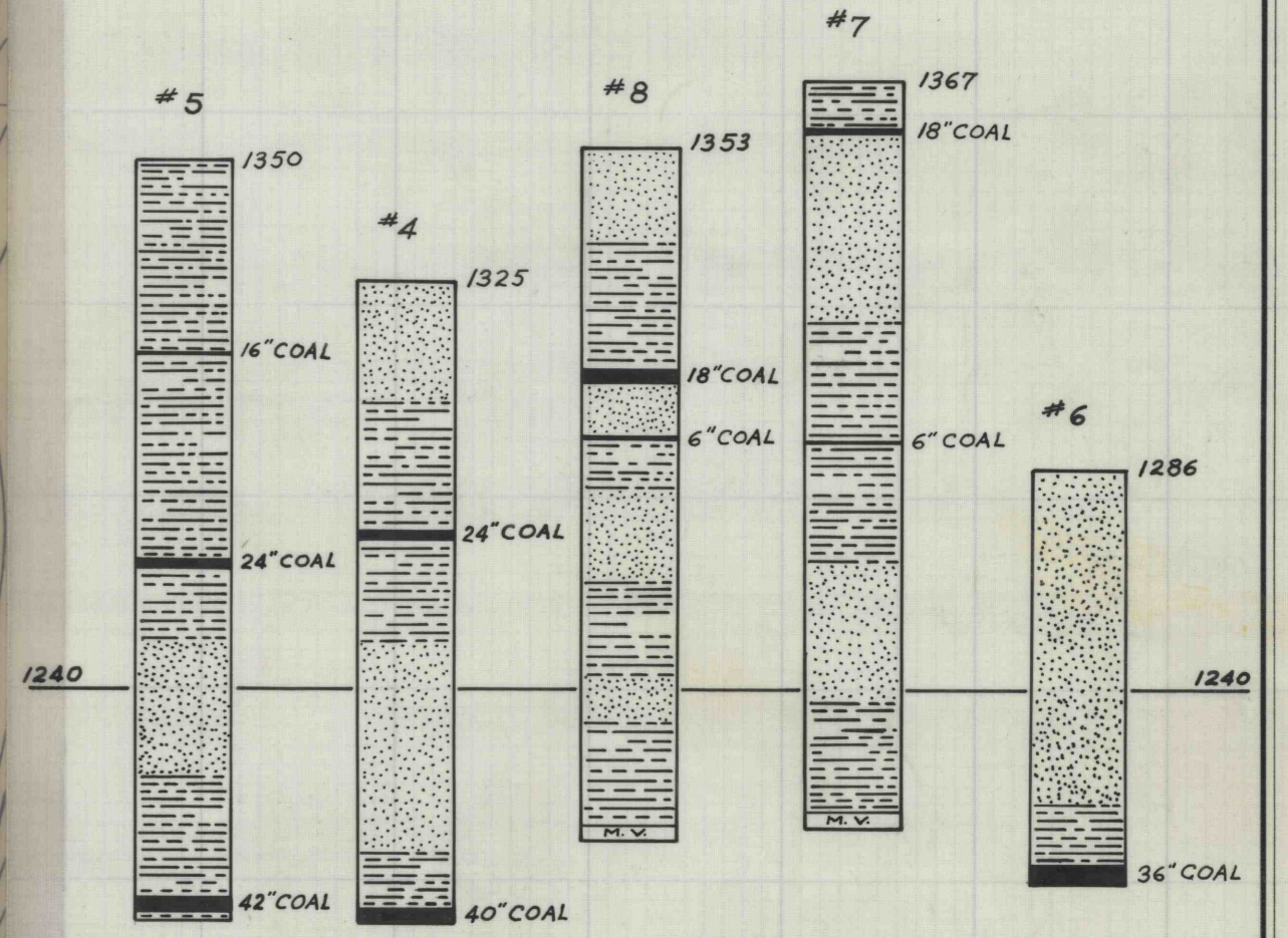
COLUMNAR SECTIONS SCALE: 1" = 40' VER.
