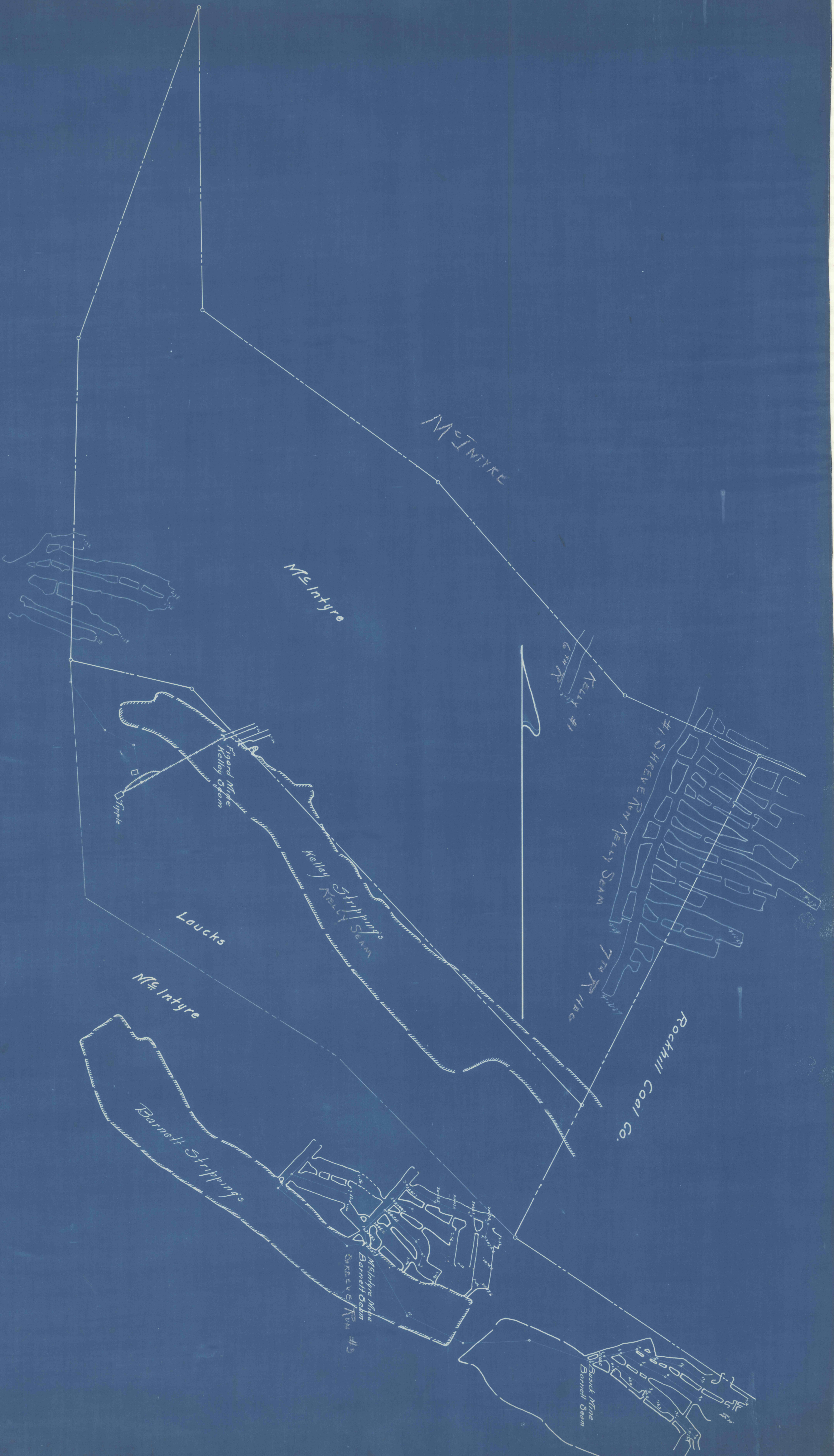
Map Showing Barnett Workings on W. McIntyre Property in Broad Top, Bedford County, Penna. July 1936 1"=100' E. Corrie Engl.
