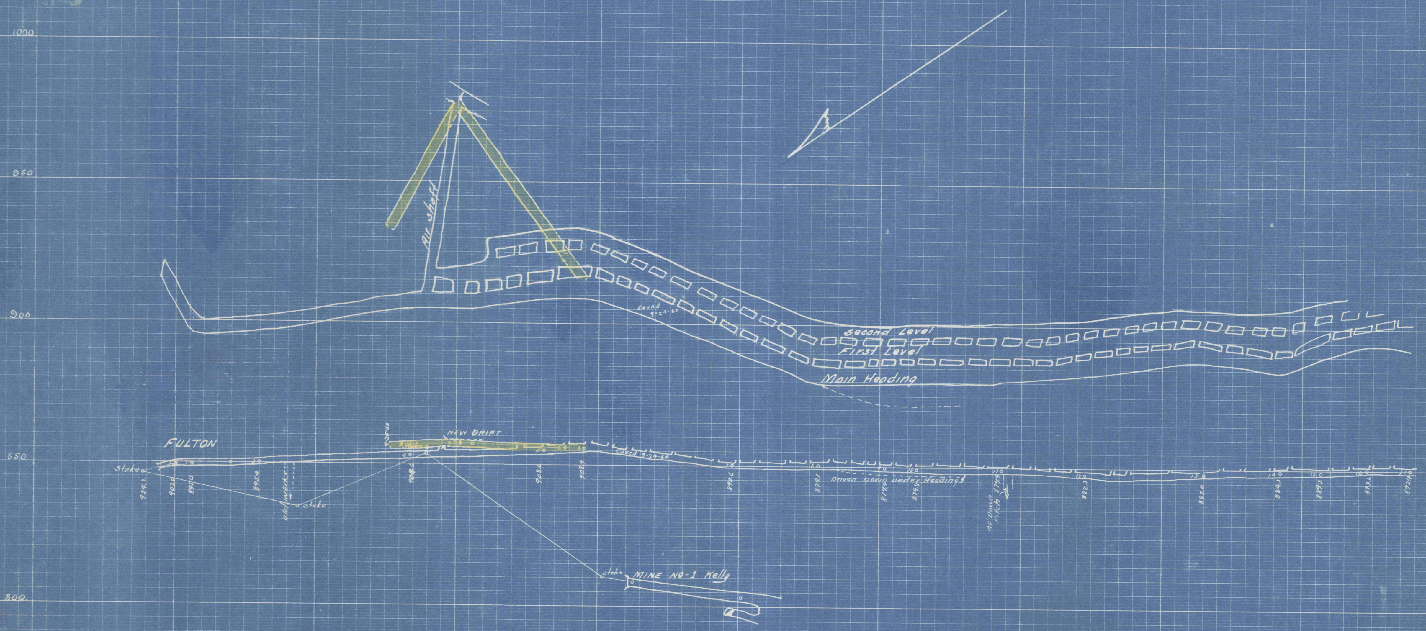
CHAS. CROTSLEY MINE MAP MINE NO 2 FULTON Rocky Ridge, Todd Twp., Hunt Co., Pa. Scale 1" = 100' Horiz. 1" = 20' Vert. March 1 st 1943 E. Corrie Engr.
