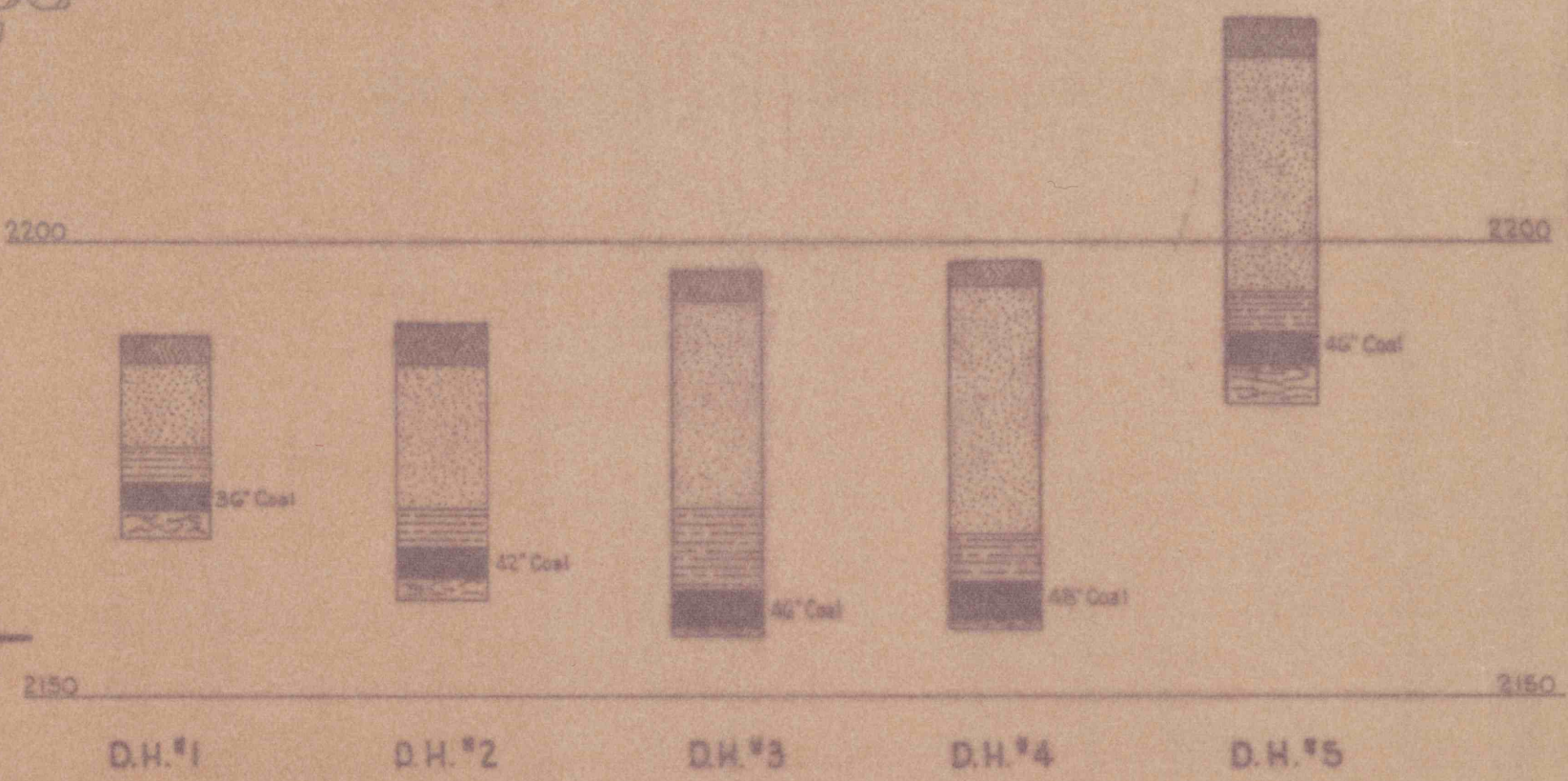
COLUMNAR SECTIONS SCALE: 1"=20'
