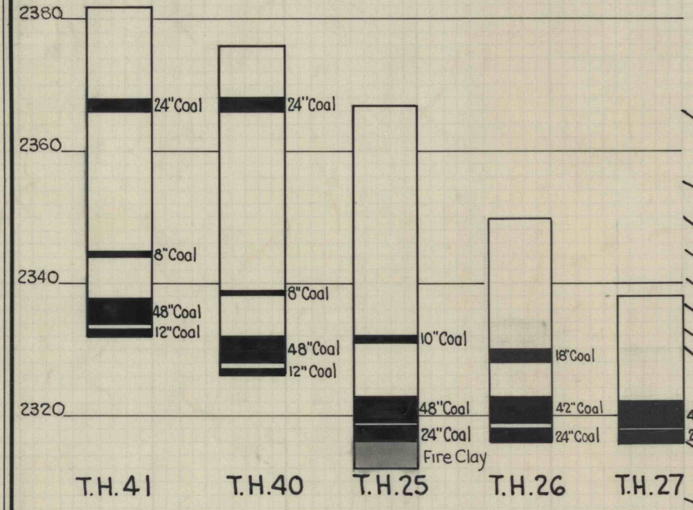
COLUMNAR SECTIONS SCALE: 1" = 20'
