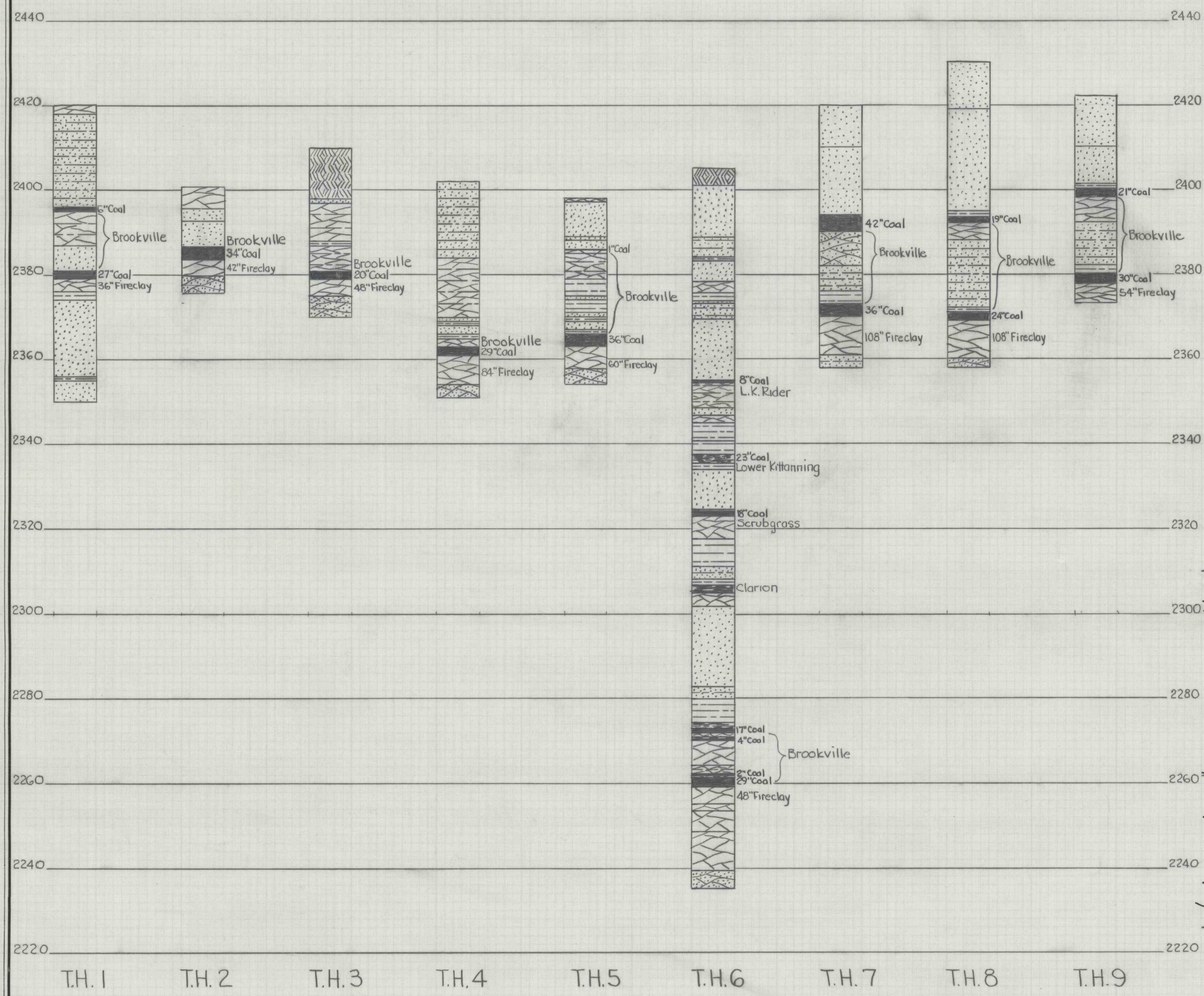
COLUMNAR SECTIONS SCALE: 1" = 20'
