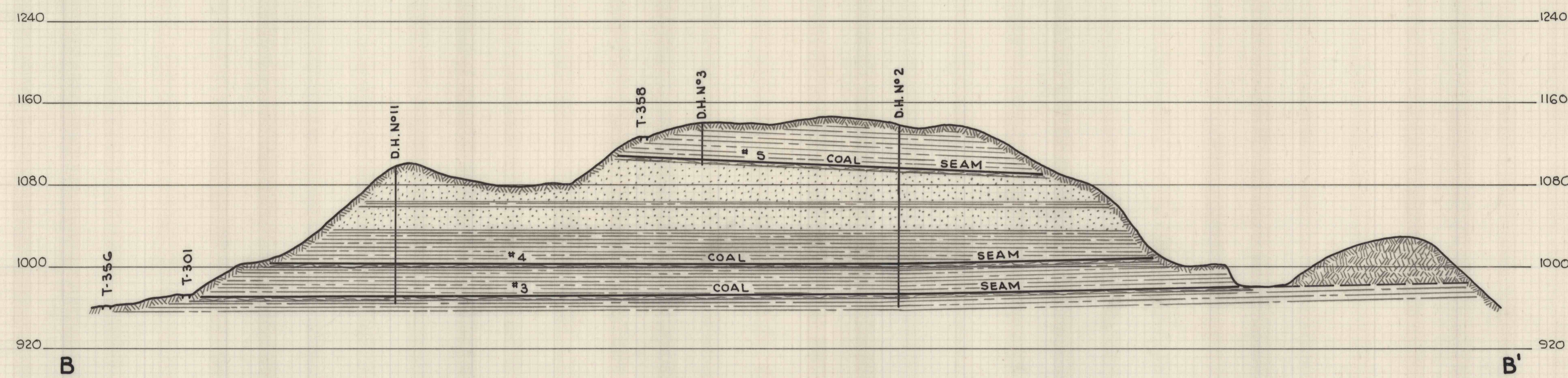
SECTION B-B'
