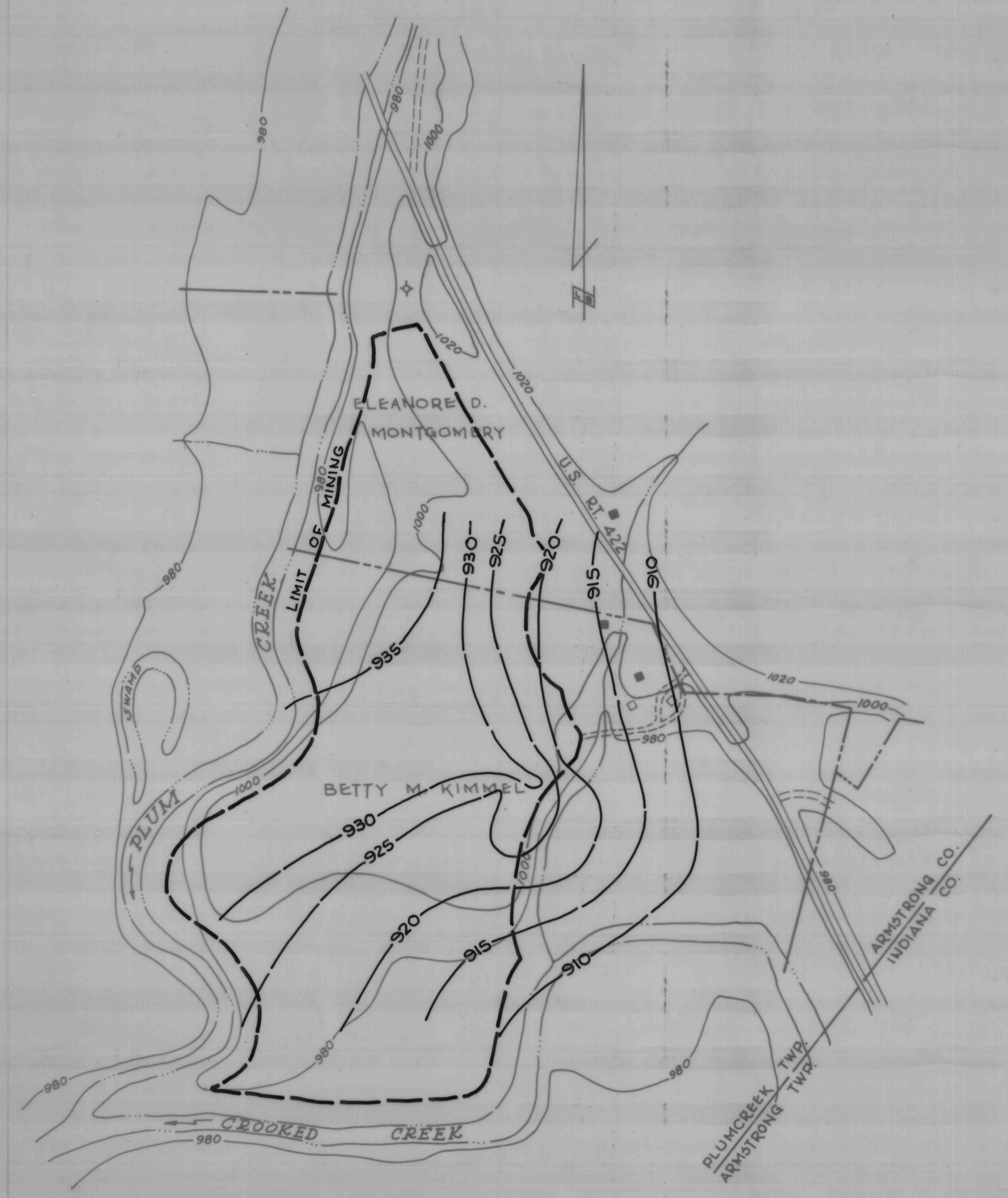
STRUCTURE MAP OF LOWER FREEPORT COAL SEAM
